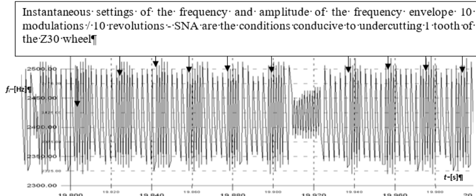
Fig. 1. Waveform of frequency as a function of time obtained from the Mi-24 sub-exciter No. 456 test No. 31, measurement No. 2 - visible temporary increase in the frequency and
