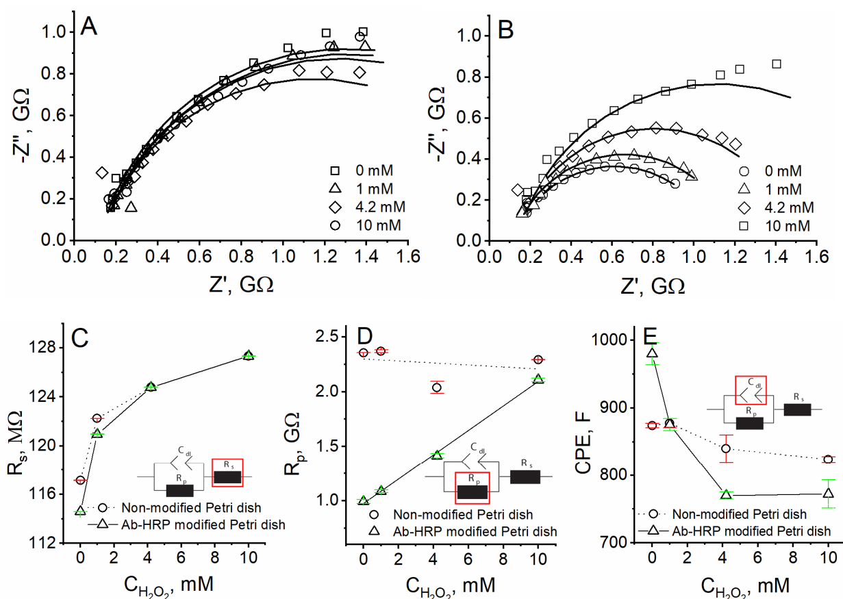
Figure 2. Nyquist plots of experiments performed at 2- \mu\text{m} distance from (A) unmodified Petri dish and (B) Ab-HRP-modified Petri dish in A-PBS with 1 mM \text{K}_3[\text{Fe}(\text{CN})_6]/\text{K}_4[\text{Fe}(\text{CN})_6] using different concentrations of \text{H}_2\text{O}_2 ; dependence of (C) resistance of solution, (D) resistance of charge-transfer, (E) double-layer capacitance on \text{H}_2\text{O}_2 concentration using unmodified and Ab-HRP-modified Petri dishes.
