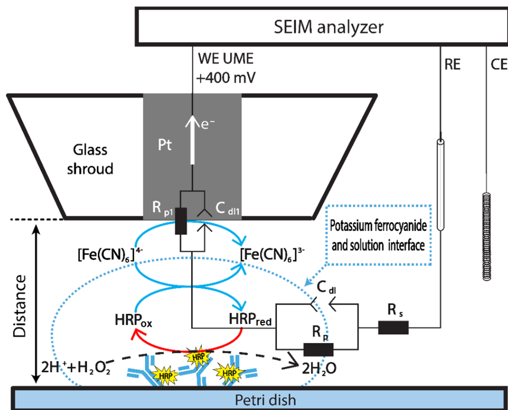
Figure 1. Schematic representation of Ab-HRP detection by EIS in the presence of potassium ferrocyanide ( \text{K}_4[\text{Fe}(\text{CN})_6] ), which serves as a redox mediator. \text{HRP}_{\text{ox/red}} —oxidized and reduced forms of horseradish peroxidase.
