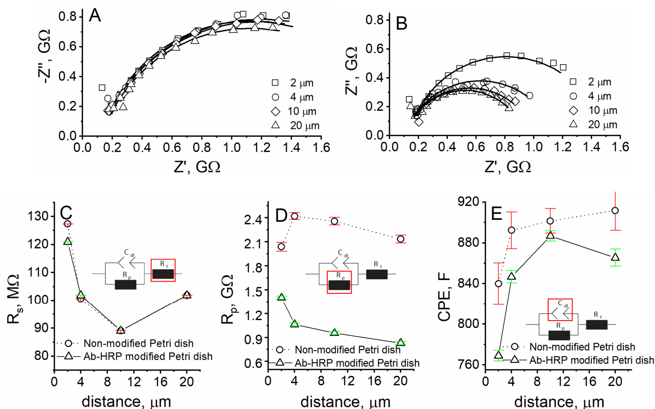
Figure 3. Nyquist plots of experiments performed at different distances from (A) unmodified and (B) Ab-HRP-modified Petri dishes in APBS with 1 mM solution of \text{K}_3[\text{Fe}(\text{CN})_6]/\text{K}_4[\text{Fe}(\text{CN})_6] using 4.2 mM \text{H}_2\text{O}_2 concentration; dependence of (C) resistance of solution, (D) resistance of charge-transfer, (E) double-layer capacitance on distance between the UME and surface of Petri dish.
