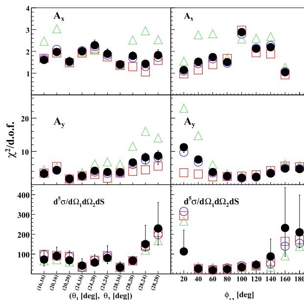
Fig. 6 The results of \chi^2/\text{d.o.f.} versus (\theta_1 and \theta_2) (left panels) and versus \phi_{12} (right panels) for different observables ( A_x , A_y and d^5\sigma/d\Omega_1 d\Omega_2 dS ) for data taken with a proton-beam energy of 135 MeV. The symbols show the theoretical calculations such as CDB (squares), CDB+ \Delta (open circles) and CDB+ \Delta +Coulomb (solid circles) and CDB+TM' (triangles). The error bars reflect the systematic uncertainty. For details, see text
