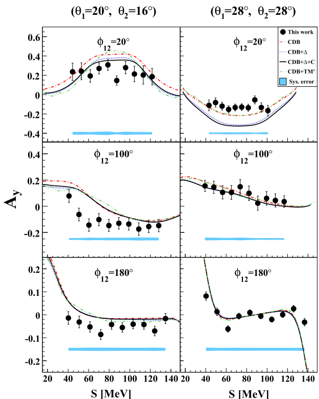
Fig. 5 The same as in Fig. 3 but for A_y
