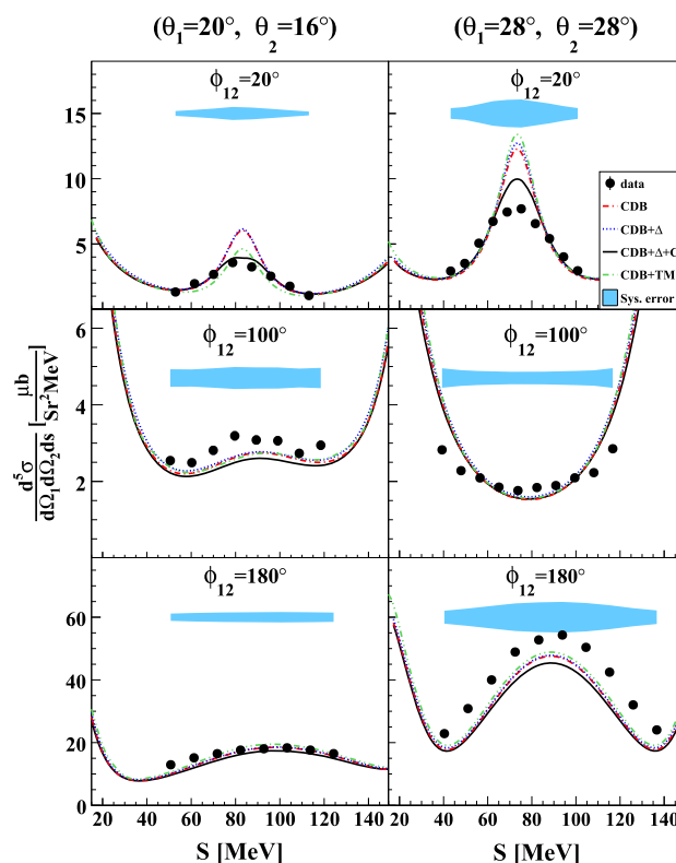
Fig. 3 Cross sections at (20^\circ, 16^\circ) (left) and (28^\circ, 28^\circ) (right) as a function of S at small, intermediate and large relative azimuthal angles for data taken with a proton beam of 135 MeV. Error bars show the statistical uncertainties for the data points. The red (dotted-dashed), blue (dotted), black (solid) and green (double dotted-dashed) lines show predictions of Faddeev calculations using CD-Bonn, CDB+ \Delta , and CDB+ \Delta +Coulomb and CDB+TM' calculations [15–18,20,40–42], respectively. The cyan bands depict the systematic uncertainties ( 2\sigma )
