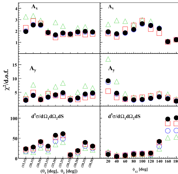
Fig. 7 Same as Fig. 6 except for 190 MeV
