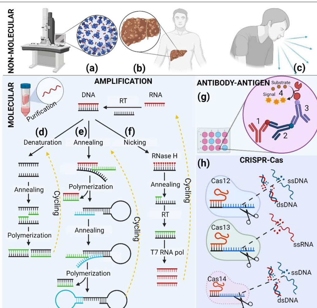
Fig. 3 Differences between molecular and non-molecular detection methods. The main application of non-molecular detection is to study the morphology ( a electron microscopy) of the viruses or to determine ( b X-ray detection) the symptoms of the viral ( c visual symptoms detection) disease. However, in molecular diagnostics, a nonspecific reaction (cutting, multiplication, amplification, etc.) or other changes must occur after the target reaction. If the method is not nonspecific, such reactions use additional components that play the role of non-specificity. Also, the purification of nucleic acids is recommended in the use of molecular applications. Nucleic acid amplification increases the amount of DNA or RNA by cyclical repeating of some procedures. In the case of PCR, real-time PCR ( d ), and loop-mediated isothermal amplification (LAMP) ( e ) methods, both a DNA and an RNA fragment can always be used for the analyte, and after amplification, the final product is always a large amount of DNA. However, nucleic acid sequence-based amplification (NASBA) ( f ) applies only to RNA detection, and the uniqueness of the method, that after the cyclic reaction, contains DNA and RNA fragments in the mixture. An enzyme-linked immunosorbent assay (ELISA) is a method that uses a solid-phase-type enzyme-linked enzyme to detect a ligand in a liquid sample using antibodies directed against the protein being measured. The ELISA method is based on a stepwise, sandwich-based combination: 1—capture antibody; 2—antibody detection; 3—secondary antibody conjugation; 4—enzymatic conversion from enzyme to colorimetric or photoluminescence substrate signal. However, fluorescent ELISA usually utilizes secondary antibodies conjugated with a fluorophore. The only drawback is the multilevel application. h Cas12, Cas13, and Cas14 are members of proteins used in CRISPR diagnostics. Cas12, Cas13, and Cas14 proteins are on the larger side of the CRISPR diagnostic protein. Cas12 and Cas14 proteins bind directly to the recognized he protospacer adjacent motif (PAM) site and cleave specified DNA sequences. After target cleavage, the Cas12 and Cas14 proteins begin to shred single-stranded DNA nonspecifically. The differences between Cas12 and Cas14—are the size of the protein and RNA length for target binding. The Cas12 protein is 1300 amino acids, and the Cas14 protein is approximately 400–700 amino acids in length. Cas12 DNA targets using 42–44 bp—however, Cas14 protein 140 bp RNA molecules length. The shorter protein spends, the fewer resources are required to obtain the Cas14 protein in the laboratory, and the more extended RNA molecular sequence of the target indicates more excellent fit and accuracy but higher costs. In RNA detection, the technique must combine Cas12 and Cas14-based diagnostics with proteins that convert RNA to DNA. The Cas13 protein directly binds and cleaves specified RNA sequences, and protein can directly detect RNA but not DNA. The Cas13 protein is 1400 amino acids in length, and the RNA guide molecule is relatively short at ~64 bp. Thus, more resources are needed to produce Cas13-based detectors, additional Cas13 does not have strict application restrictions, but RNA targets can accept structures that are difficult to cut due to structural limitations. More detailed differences are given in separate article sections and Table 1
