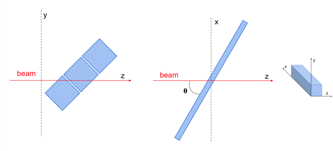
Figure 19. Sketch of the LYSO:Ce bars orientation with respect to the beam in two configurations: transverse cross section of the bars for a rotation in the yz plane (left); rotation in the xz plane with the beam forming an angle of incidence \theta with respect to the bar longitudinal axis (right).
