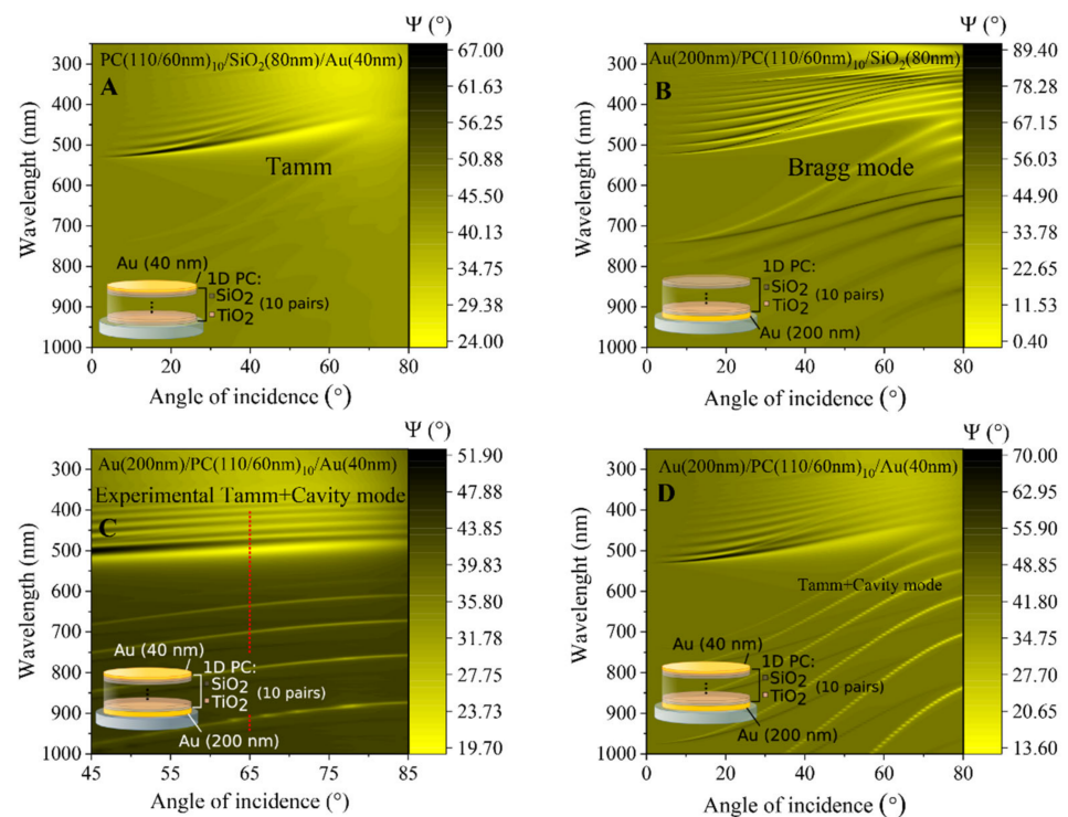
Figure 3. Dispersion relations of calculated TPP (A), cavity mode (B), TPP + CM (D), and an experimental dispersion of the investigated modified QCM-D sensor chip, supporting TPP and CM (C). Red dashed line in (C) marks a cross-section at \theta_i = 65^\circ .
