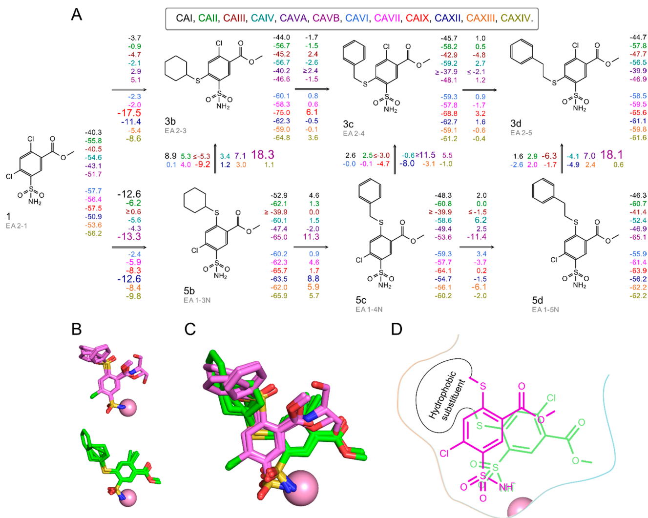
Figure 4. Correlation of compound chemical structures with the changes in standard intrinsic Gibbs energy upon binding and comparison of the crystal structures between CA isozymes. (A) Differences of \Delta G_{intr} (kJ/mol) between neighboring compounds are listed on the connecting arrows. Colors represent CA isozymes. (B) Superimposed ligands of these crystal structures: (upper panel) para -substituted ligands are colored magenta: CAXII—3b (PDB ID: 7PP9), CAXII—3d (PDB ID: 7PUW), CAIX—3b (PDB ID: 7POM), mimic-CAIX—3b (PDB ID: 7Q0C), (lower panel) ortho -substituted ligands are colored green: CAXII—EA3-3 (PDB ID: 6R6F), CAXII—EA3-2o (PDB ID: 6R71), CAXII—5b (PDB ID: 7PUU), CAXII—9a (PDB ID: 7PUV), CAII—9a (PDB ID: 7Q0E). (C) The abovementioned superimposed structures are shown for comparison. (D) Scheme representing compound position shown in panel C. Orange line represents more hydrophobic side of the active site. Zinc ion is shown as a pink sphere.
