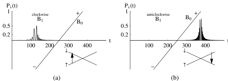
Figure 1. The probability P_{\downarrow}(t) to find the spin in the down direction when the magnetic field \mathbf{B}_0 = B_0 \mathbf{e}_3 linearly increases from B_0 = -2 to B_0 = 2 in the time interval T = (t_{\text{fin}} - t_{\text{ini}}) = 500 . The exciting field \mathbf{B}_1 that flips the spin from \uparrow to \downarrow direction, as shown in the insets by long vertical arrows, is rotating in \mathbf{e}_{12} -plane: clockwise in (a) and anticlockwise in (b). The insets show the up and down spin eigenenergies as a function of magnetic field strength. In (a) the absorption and in (b) the stimulated emission take place that are the main processes that determine performance of a laser, which is the acronym of “light absorption [and] stimulated emission [of] radiation”. Other parameters in the calculation: \omega = 1 , \omega_1 = 0.05 .
