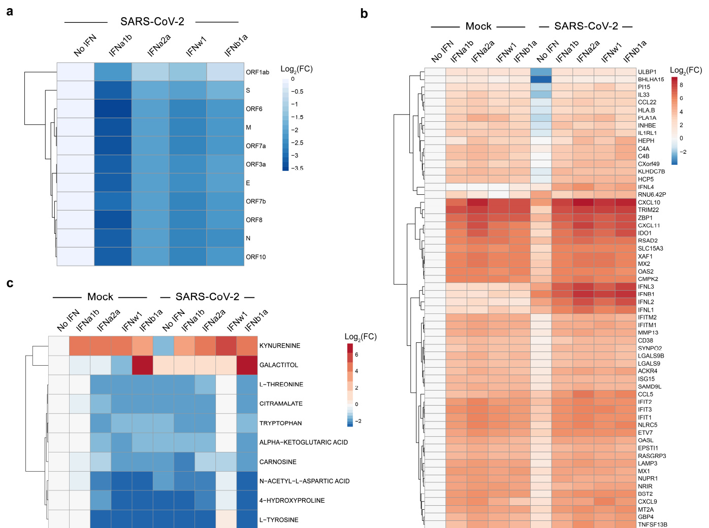
Figure 4. Transcriptomic and metabolomic analyses of mock- and SARS-CoV-2-infected Calu-3 cells, non-treated or treated with type I IFNs. (a) Calu-3 cells were stimulated with IFNs (1 \mu g/mL) or non-stimulated, and infected with SARS-CoV-2 (moi = 0.01). A heatmap of viral RNAs affected by treatment is shown. Each cell is colored according to the log 2 -transformed expression values of the samples, expressed as fold-change relative to the non-treated control. (b) Calu-3 cells were either stimulated with recombinant human IFN (1 \mu g/mL) or left untreated with IFN, then infected with either mock or SARS-CoV-2 (moi = 0.01). A heatmap of the most variable cellular genes affected by treatment and virus infection is shown. Each cell is colored according to the log 2 -transformed expression values of the samples, expressed as fold-change relative to the non-treated, mock-infected control. (c) Cells were treated as for panel b. After 24 h, the cell culture supernatants were collected, and metabolite levels were determined by LC-MS/MS. A heatmap of the most-affected metabolites is shown. Each cell is colored according to the log 2 -transformed profiling values of samples, expressed as fold-change relative to the mock control.
