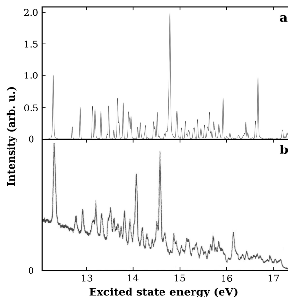
Figure 1. Simulated (a) and measured (b) [2] spectra of Auger electrons ejected from 5p -core excited states of Cs excited by 30 eV electron-impact.
