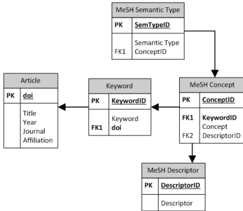
Fig. 40. Entity-relationship diagram of the relational dataset
