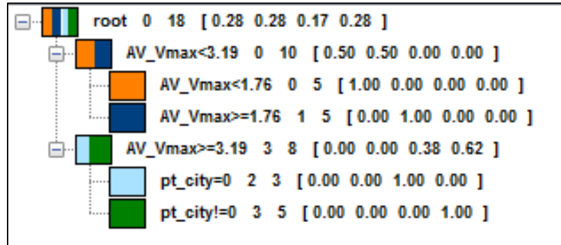
Fig. 34. Aortic stenosis grading decision tree based on cardiologist measurements
