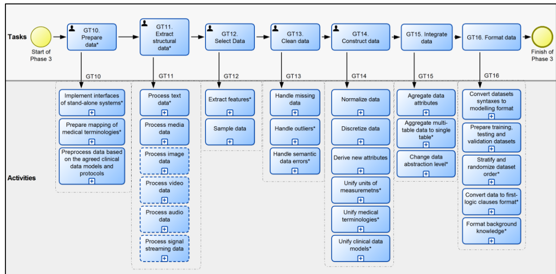
Enhanced activities are marked with * Fig. 15. Phase 3 “Data Preparation” general tasks and activities.
