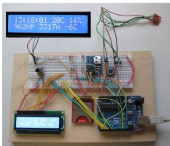
Figure 1: Weather station
