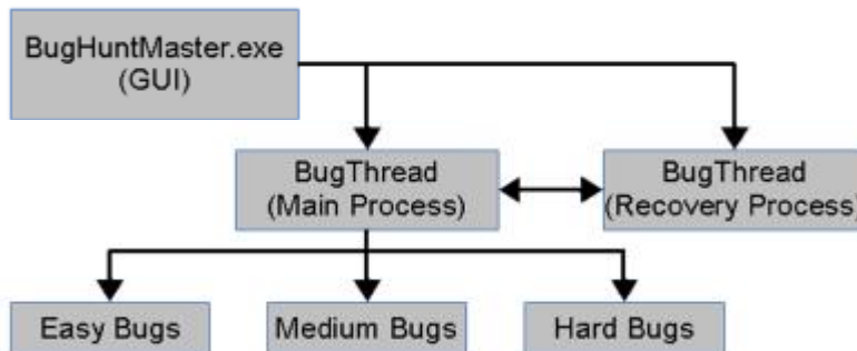
Figure 1: Sketch of the BugHunt architecture
