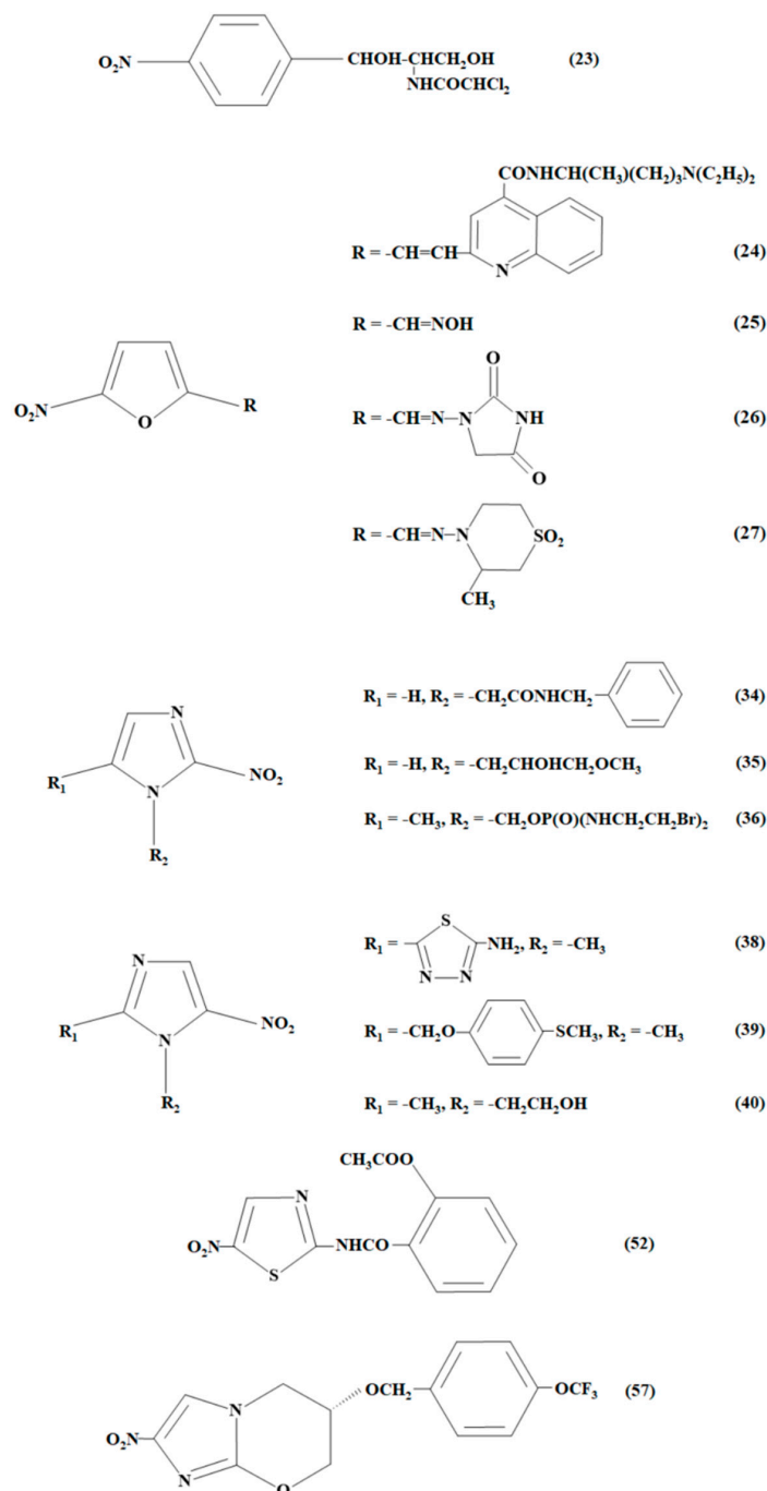
Figure 1. Formulas of nitroaromatic antibacterial and antiparasitic agents: chloramphenicol (23), chinifur (24), nifurxime (25), nitrofurantoin (26), nifurtimox (27), benznidazole (34), misonidazole (35), TH-302 (36), megalzol (38), fexinidazole (39), metronidazole (40), nitazoxanide (52), and PA-824 (57). The numbers of compounds correspond to those in Table A1 (Appendix A).
