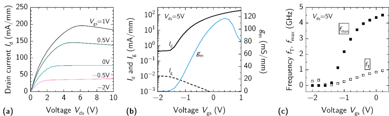
Figure 8. (a) Output characteristics, (b) transfer characteristics and (c) f_T and f_{max} frequencies measured for the same HEMT with L_g = 5 \mu m and L_{ds} = 12 \mu m.
