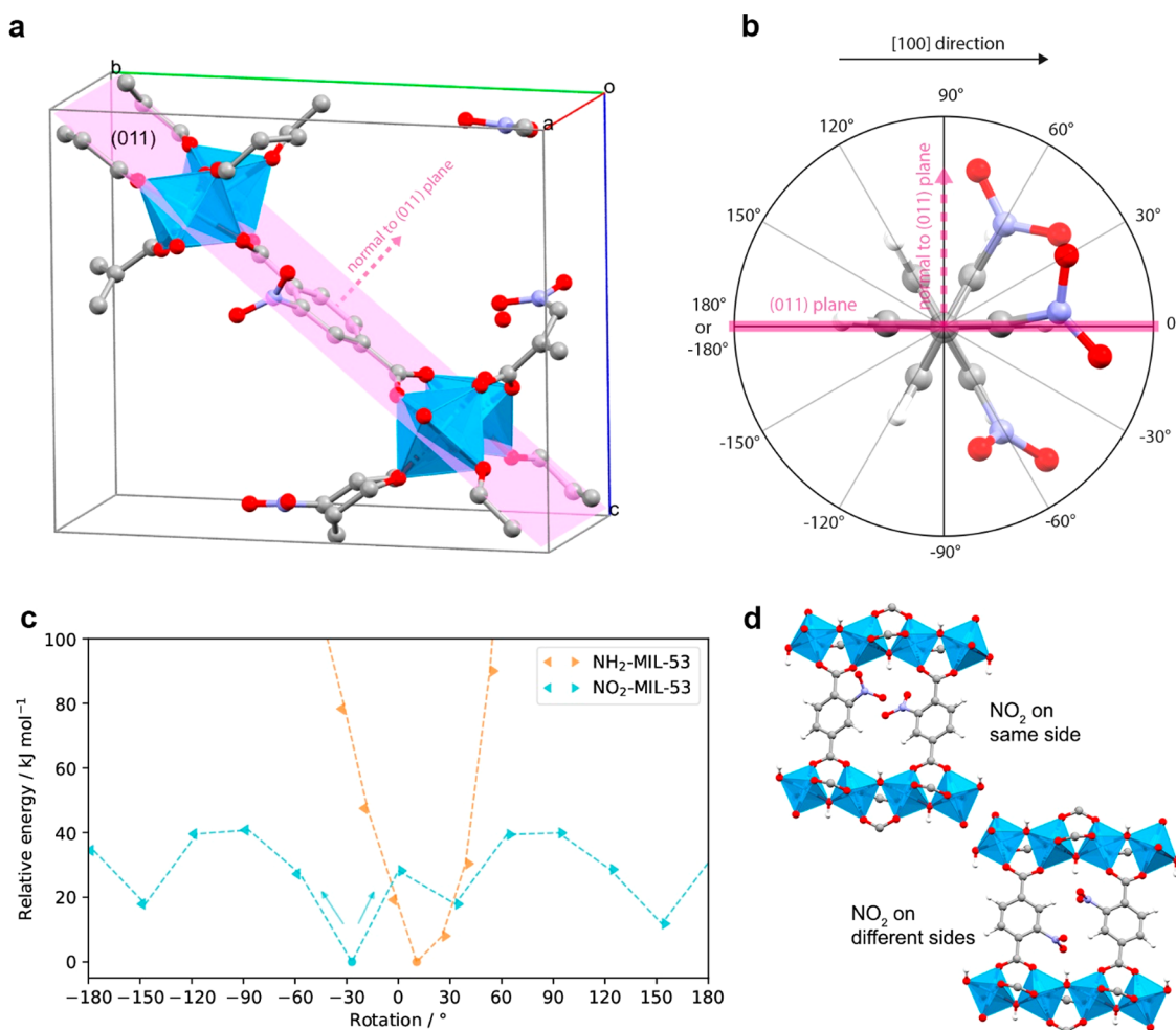
Figure 2. Effect of linker rotation on the potential energy as studied by DFT. (a) Unit cell of \text{NO}_2\text{-MIL-53(Al)} with central linker in 0^\circ rotation with respect to (011) plane (pink); hydrogens omitted for clarity. (b) Rotation angle is defined as the angle between benzene ring plane and (011) plane, taking 0^\circ as the conformation with the functional group pointing in the positive [100] direction. The sign of the angle is assigned based on the direction normal of the reference plane. (c) Potential energy profiles for the rotation of one linker in a \text{NH}_2\text{-MIL-53(Al)} and \text{NO}_2\text{-MIL-53(Al)} unit cell. The direction of rotation is indicated by the direction of the marker. (d) Example of an unfavorable head-to-head nitro group encounters in adjacent linkers when they are located on the same side of the ring (top) and on different sides (bottom).
