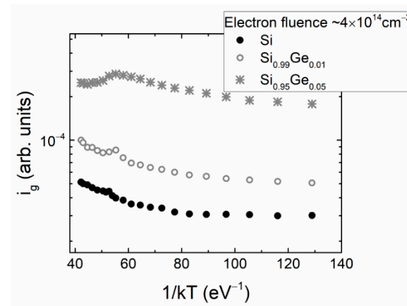
Figure 6. Generation current variations as a function of the inverse thermal excitation energy measured in samples under IR laser illumination.
