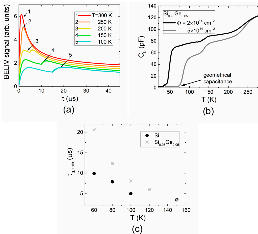
Figure 4. (a) Simulated variations (using Equations (1) and (3)) of the BELIV transients assuming changes of material resistivity, concentration of injected carriers, as well as minority and majority carrier traps of different generation lifetime. (b) Temperature-dependent barrier capacitance ( C_b ) variations in diodes containing different concentration of radiation-induced traps, where C_b approaches a geometrical value due to full extraction of thermally emitted carriers. (c) Minority carrier thermal generation lifetime as a function of temperature measured by BELIV technique in p -type Si and SiGe alloy.
