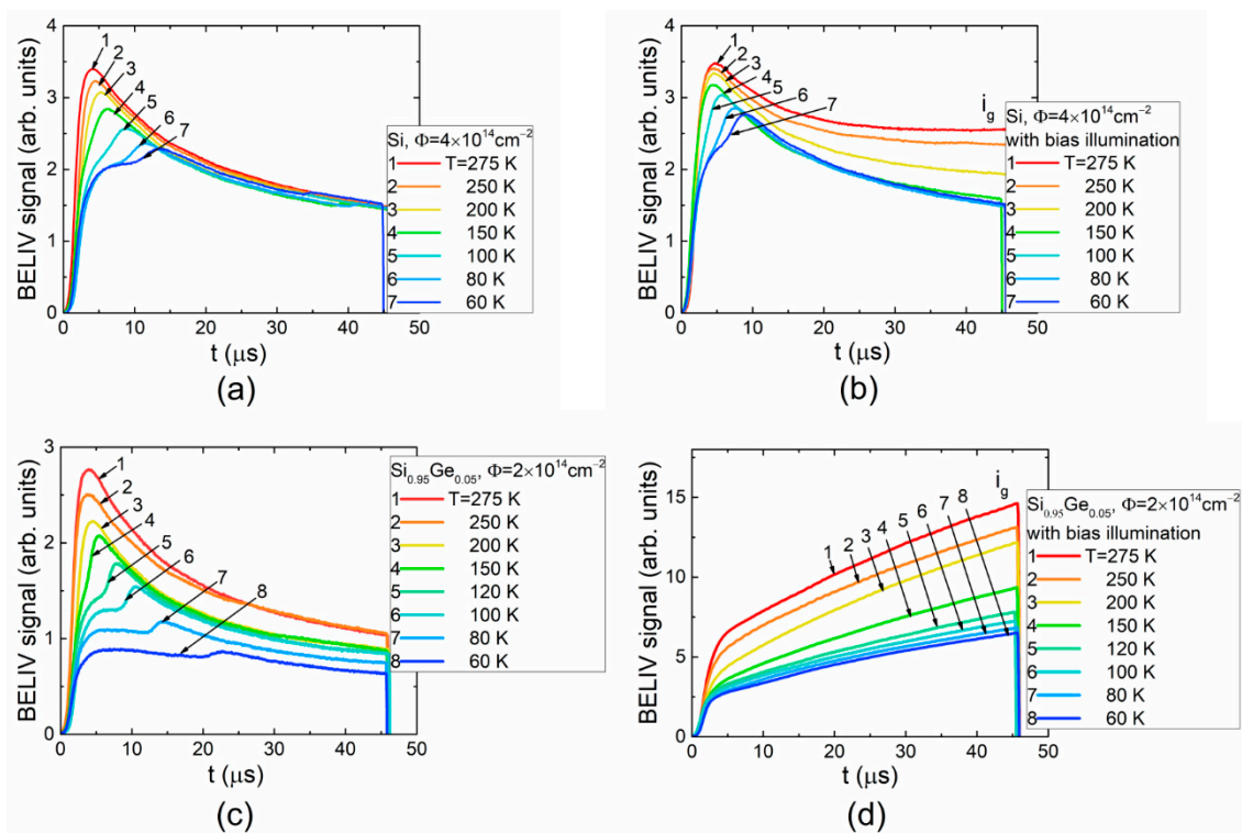
Figure 3. (a–d) Temperature-dependent BELIV transients in Si and \text{Si}_{1-x}\text{Ge}_x diodes measured in dark (a,c) and under (b,d) laser illumination.
