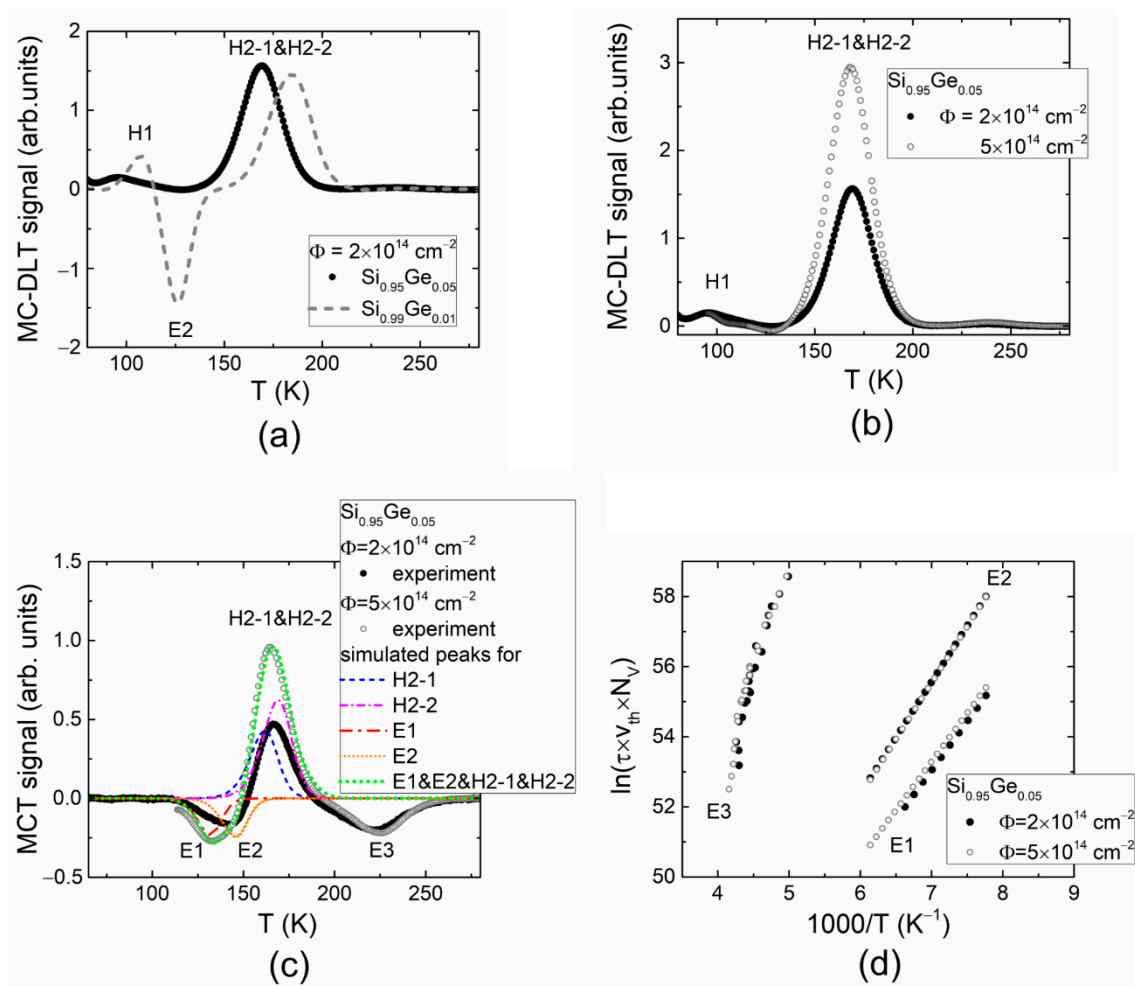
Figure 2. (a) Comparison of the MC-DLT spectra recorded by electrical injection of the excess carriers in the 2 \times 10^{14} \text{ cm}^{-2} fluence electron-irradiated \text{Si}_{0.99}\text{Ge}_{0.01} and \text{Si}_{0.95}\text{Ge}_{0.05} diodes; (b) Comparison of MC-DLT spectra recorded in \text{Si}_{0.95}\text{Ge}_{0.05} diodes irradiated with 2 \times 10^{14} \text{ cm}^{-2} and 5 \times 10^{14} \text{ cm}^{-2} fluence where only majority carrier trap associated peaks are observed; (c) Comparison of the MCT spectra recorded in \text{Si}_{0.95}\text{Ge}_{0.05} diodes irradiated with 2 \times 10^{14} \text{ cm}^{-2} and 5 \times 10^{14} \text{ cm}^{-2} 5.5 MeV electron fluence using optical injection of the excess carrier pairs. Here, the dotted curves illustrate the simulated spectral peaks ascribed to different traps. (d) Arrhenius graphs plotted for different peaks in MC-DLT and MCT spectra.
