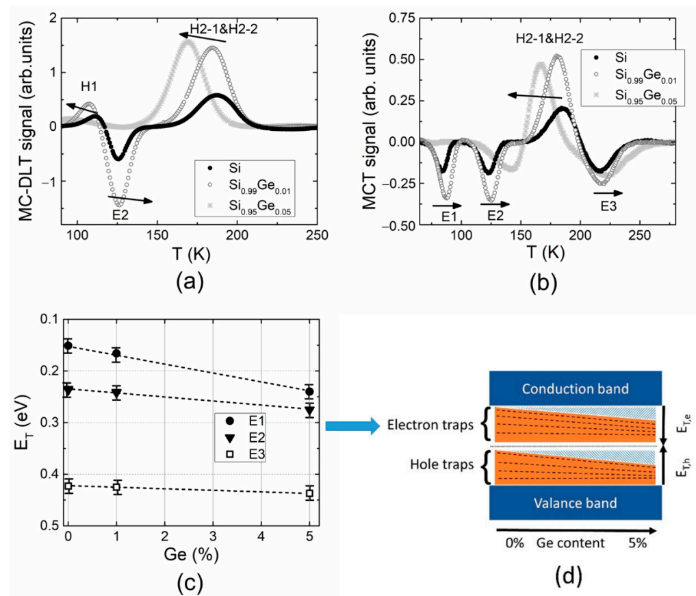
Figure 5. Comparison of MC-DLT (a) and MCT (b) spectra obtained in the 5.5 MeV electron-irradiated Si, Si 0.99 Ge 0.01 and Si 0.95 Ge 0.05 diodes; (c) The activation energy values ( E_T ) of the radiation-induced traps (E1–E3) of minority carriers as a function of Ge content; (d) A tentative scheme of the band gap variation in p -type Si 1-x Ge x material and related activation energy changes in the minority carrier traps depending on the Ge content.
