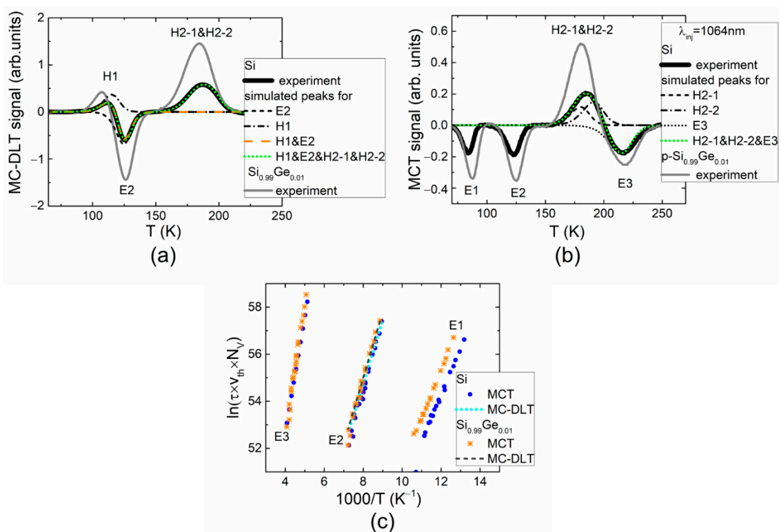
Figure 1. (a) The MC-DLTS spectra (solid curves) recorded under electrical carrier injection in 5.5 MeV electron-irradiated and boron-doped Si and Si 0.99 Ge 0.01 diodes (the dot curve represents the simulated spectrum, including all the traps inherent for the IR illuminated diode after prolonged (16 h) retention in dark (at 293 K temperature)); (b) The MCT spectra (solid curves) of the same Si and Si 0.99 Ge 0.01 diodes recorded under optical injection implemented by short IR illumination of the diode edge and prolonged (16 h) retention in dark of the illuminated sample at 293 K temperature. Here, black curves represent spectra obtained for Si, while gray curves show these spectra recorded for Si 0.99 Ge 0.01 diodes, and the dotted curves illustrate the simulated spectral peaks. (c) Arrhenius graphs plotted for different peaks in MC-DLT and MCT spectra. Here, \tau denotes carrier lifetime relative to emission; v_{th} is the carrier thermal velocity; N_V is the effective density of free carrier states.
