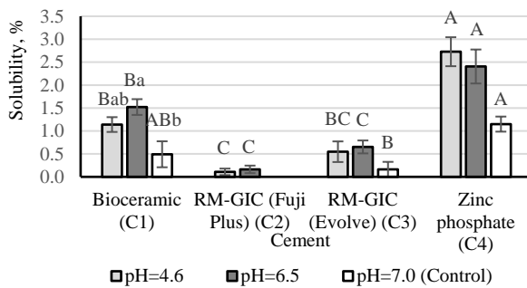
Fig. 5. Solubility after 120 (SL120) hours. Each bar shows the mean for 9 replicates \pm standard error (SE). Different letters indicate significant differences among tested cement ( P < 0.05 , Tukey's (HSD) test)
