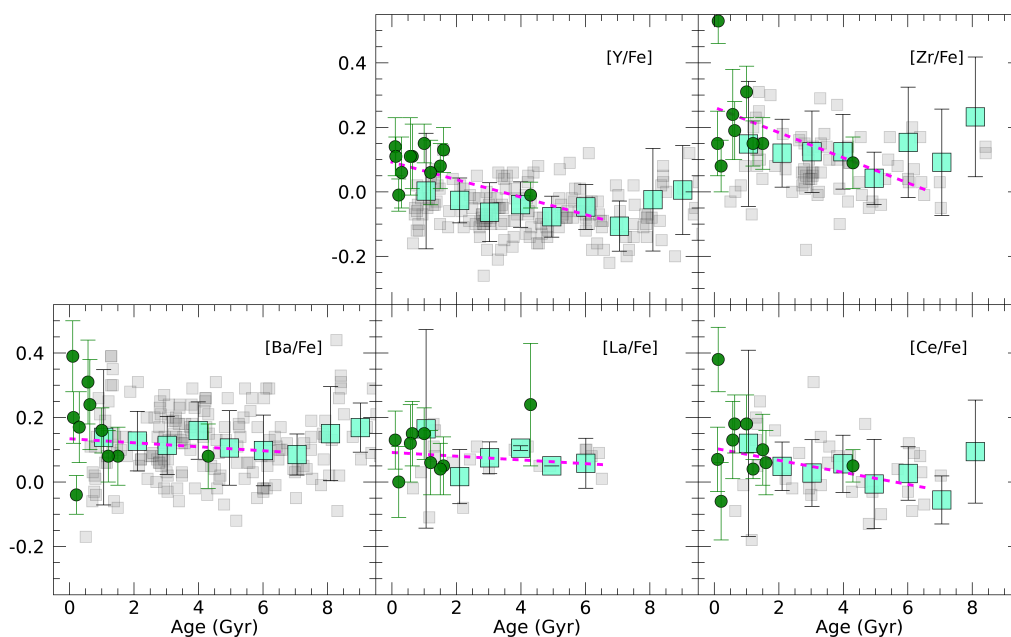
Figure 1. Abundance ratios [El/Fe] vs. age for the thin-disc stars (binned results, bin 0.1 dex wide—cyan squares, and individual stars—grey squares) and the open clusters located in the solar neighbourhood (green circles). The magenta dashed lines are the weighted linear fits to the cumulative sample of solar neighbourhood clusters and thin-disc field stars for stellar ages <8 Gyr (figure adapted from [29]).
