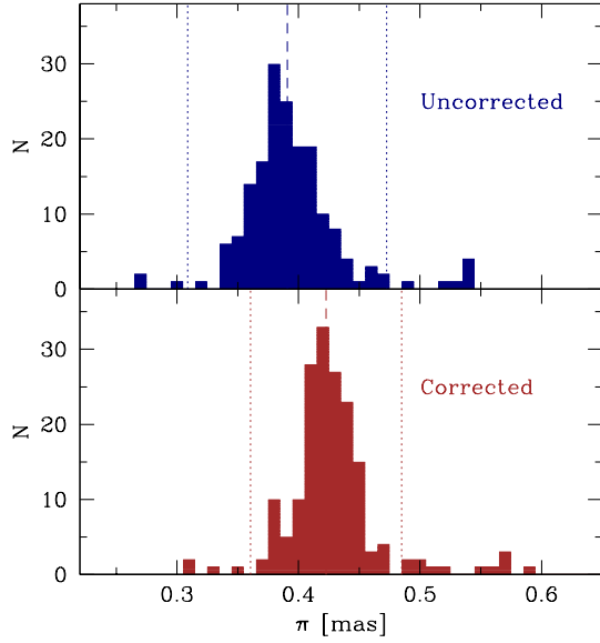
Fig. 1. Breakdown of the parallaxes for the stars with well-behaved astrometric solutions before ( top panel ) and after ( bottom panel ) applying the zero-point offsets of Lindegren et al. (2021a) . A foreground star (GES 10344563–5813091) with a much larger parallax is off scale. The dashed lines show the mean values, while the dotted lines indicate the 3\text{-}\sigma thresholds.
