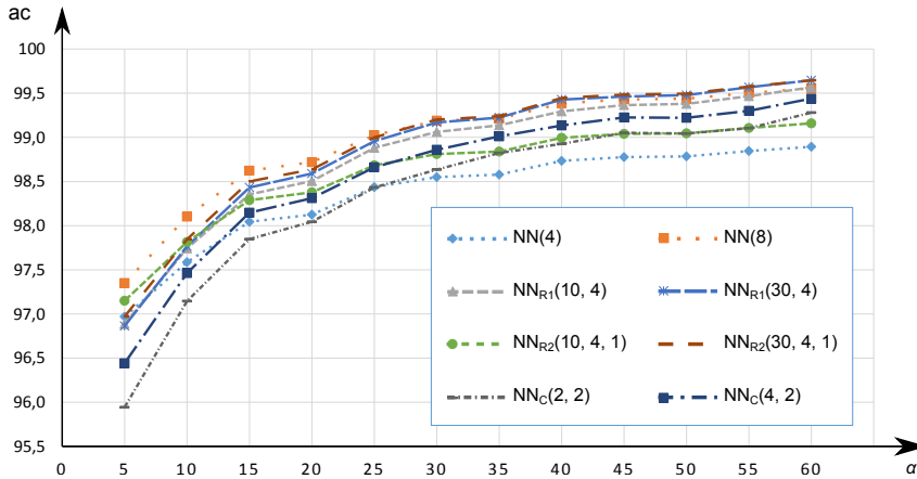
Fig. 3. Results of the classification accuracy (ac) using SCR D classification method with different neighborhood schemes. Results are presented according to different correlation range parameter \alpha values.
