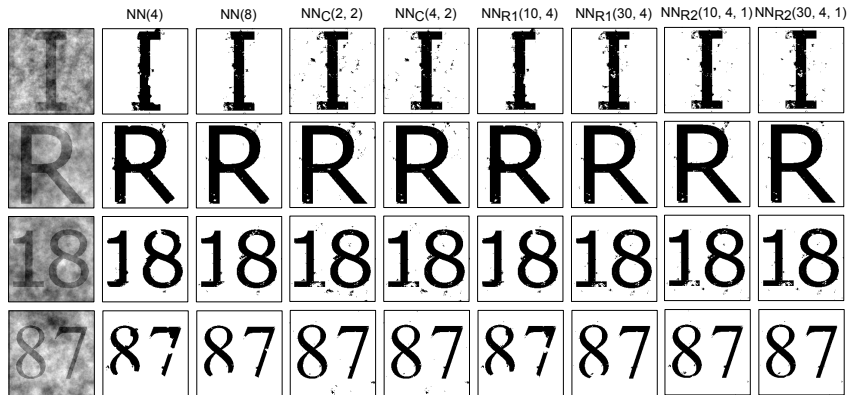
Fig. 4. Visual results of the classification. Most interesting images are presented.
