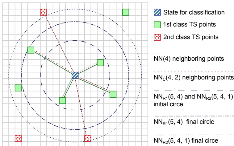
Fig. 1. Examples of neighborhood schemes used in this letter.
