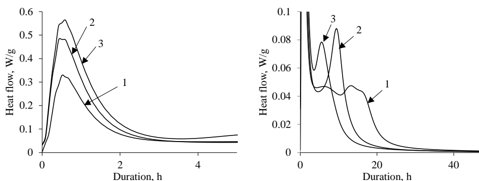
Fig. 1. The heat evolution rate of mayenite and gypsum mixture, curves: 1 – CA1_2.5, 2 – CA1_5 and 3 – CA1_7.5 samples during the early stage of hydration (a water/solid ratio of 0.75).
