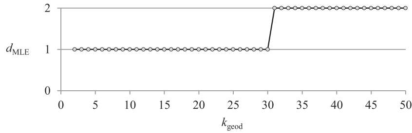
Fig. 23. Estimate d_{MLE} of the intrinsic dimensionality depending on the number k_{geod} of the nearest neighbours in the calculation algorithm of geodesic distances; data set: the helix.
