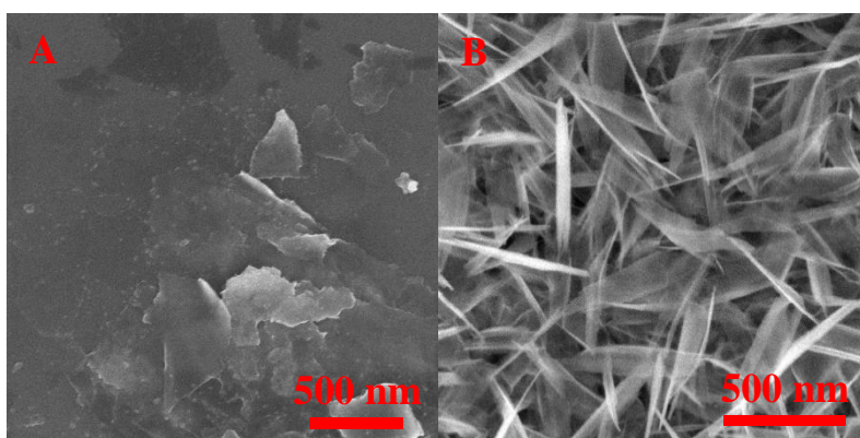
Fig. 1. SEM images of A – MXenes ( \text{Ti}_3\text{C}_2\text{T}_x ) sheets, B – \text{TiO}_x nanostructures.
