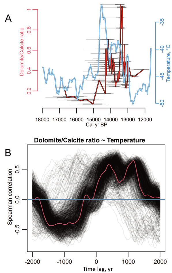
Fig. 6. Analysis of statistical correlations between dolomite/calcite ratios in the Zervynos-2 lower gyttja section, and GISP2 temperature data: A – time series of dolomite/calcite ratio (red) and GISP2 temperature (light blue). The red line represents the average dolomite/calcite ratio time series, whose samples were assigned the average dates from the BAD model posterior distributions. The horizontal bars depict the probability intervals (PI) of the date of each sample (narrow bars: 2–98% PI, medium bars: 6–94% PI, wide bars: 16–84% PI). B – curves of cross-correlation between dolomite/calcite ratio and GISP2 temperature. Each black curve represents a different iteration of the BAD model, and the red curve – the mean BAD model. The horizontal blue line separates positive and negative correlations. Positive time lag values mean that the carbonate time series were shifted back in time and vice versa. A high correlation at positive lag values shows the delayed response of carbonate compositions to climate change, as measured in GISP2.
