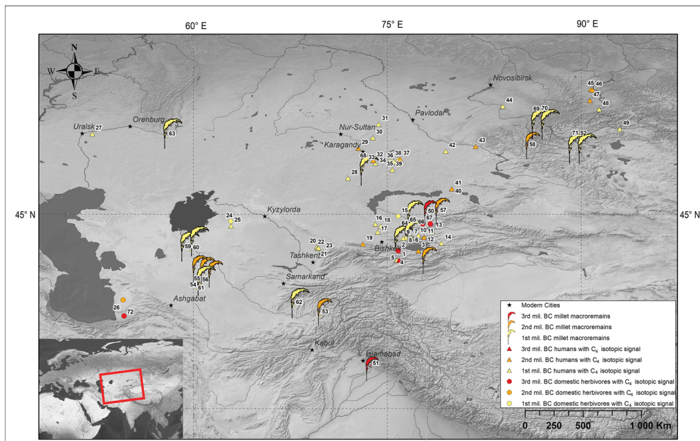
Figure 7. The distribution of broomcorn millet ( Panicum miliaceum ) macroremains and C_4 plants consumers outside China (for detailed references, see the online supplementary material (OSM D)) (figure by the authors).
