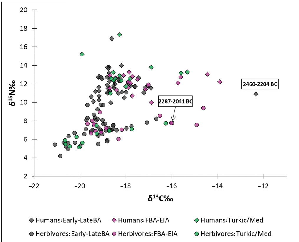
Figure 2. Scatter plot of stable isotope values of human and animal bone collagen from Kyrgyzstan (BA = Bronze Age; FBA = Final Bronze Age; EIA = Early Iron Age) (figure by the authors).
