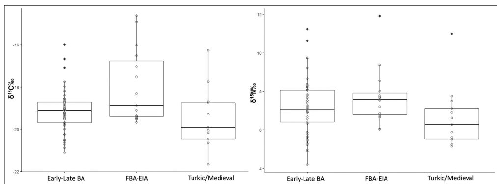
Figure 5. Box plots showing the variation of animal isotopic values through time (figure by the authors).
