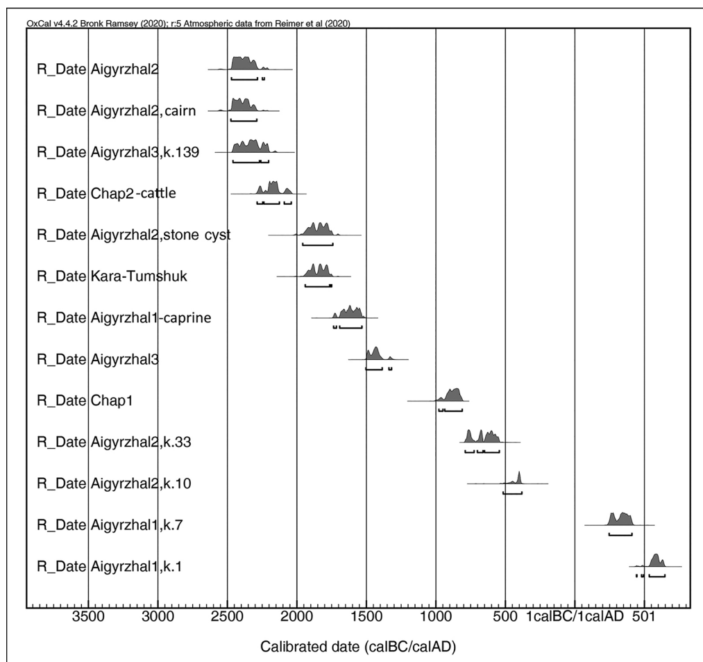
Figure 3. OxCal v4.4.2 calibration curves of the human and faunal bone dates from Kyrgyzstan (dates calibrated in Oxcal v4.4.2 using the IntCal20 atmospheric curve; Bronk Ramsey 2020; Reimer et al. 2020).
