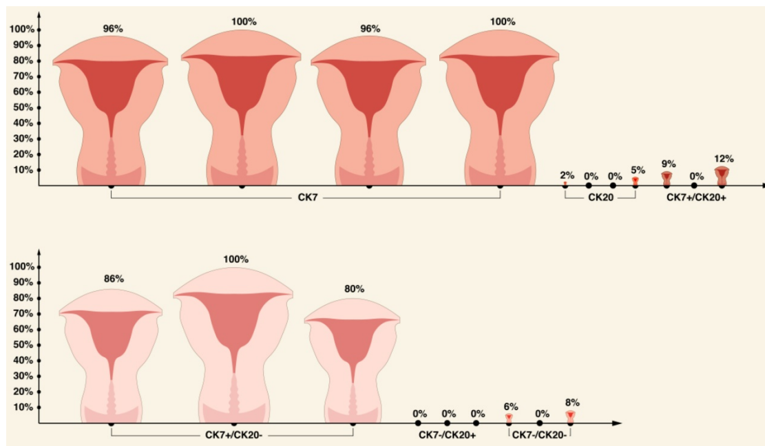
Figure 4: Comparison of CK7 and CK20 expression in EC based on literature review [56, 62, 75-77].
