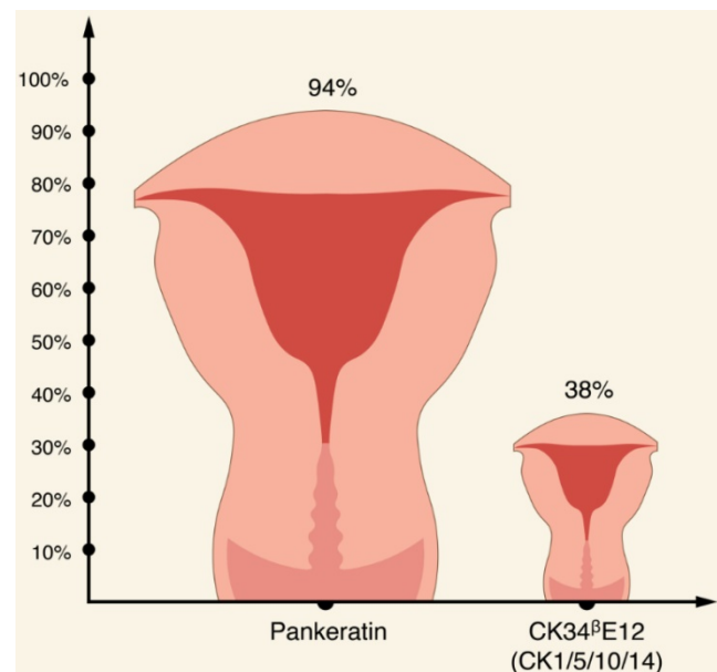
Figure 3: Comparison of the expression patterns of pankeratin and CK1/5/10/14 in ECs [76-77].
