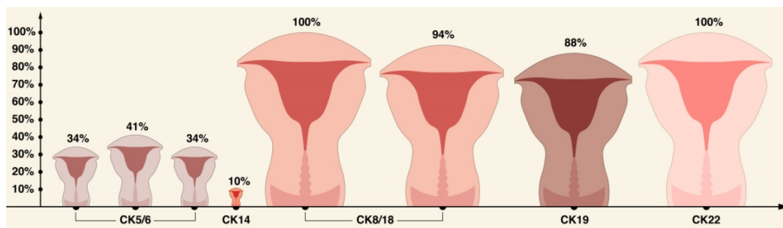
Figure 5: Comparison of CK5/6, CK14, CK8/18, CK19, and CK22 in ECs based on literature review [56, 69, 76].
