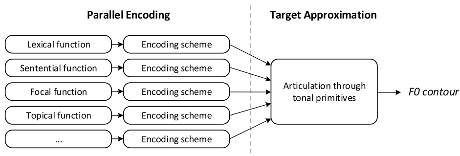
Fig. 7. PENTA model.
