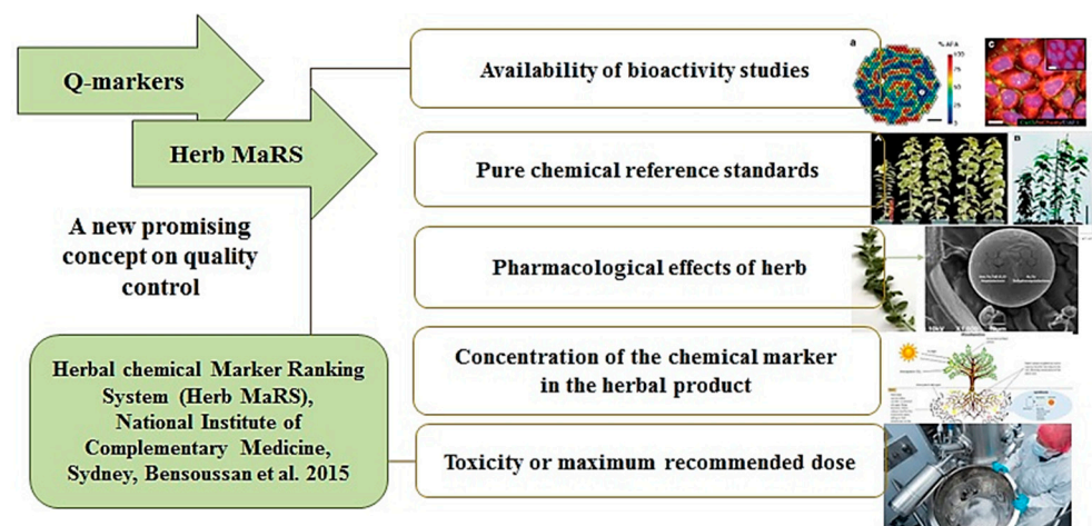
Figure 4. Herb MaRS criteria for chosen of Q-markers for Crocus perianth raw material and crude extracts.
