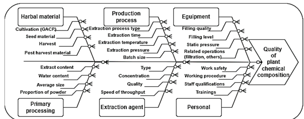
Figure 2. Risk assessment of C. sativus perianth extracts obtaining using the Ishikawa method.
