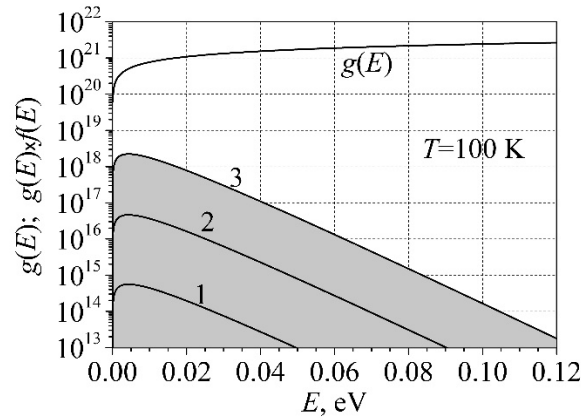
Figure 4. The conduction band state filling function g(E)f(E) dependence on energy for three phosphorous doping densities, in \text{cm}^{-3} : 1— 10^{13} ; 2— 10^{15} ; 3— 10^{17} . The densities of electrons below the curves are equal to the ionized phosphorous donor densities.
