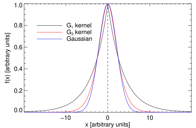
Fig. C.1: Shapes of the kernels G_1 and G_3 in comparison with a Gaussian. For display purposes all functions were normalised to G_i(0) = 1 . All share the same FWHM.
