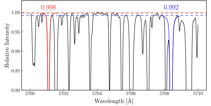
Fig. 3. Comparison of two silicon line profiles while locally fitting the continuum. Observations are shown in black and the fitted syntheses at 5701.11 and 5708.40 \text{ \AA} are shown in red and blue, respectively, along with the fitted continuum value. Across a wider wavelength range, the various fitted continua are not consistent with one another.
