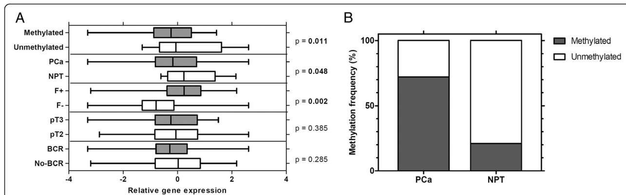
Fig. 3 Expression levels (a) and methylation frequency (b) of ABCB1 in prostate tissues. PCa – prostate cancer; NPT – noncancerous prostate tissue; BCR – biochemical recurrence; F +/− – TMPRSS2-ERG fusion status. The box of figure A extends from the 25 th to the 75 th percentiles. The line in the middle of the box is plotted at the median. The whiskers indicate the smallest and largest values
