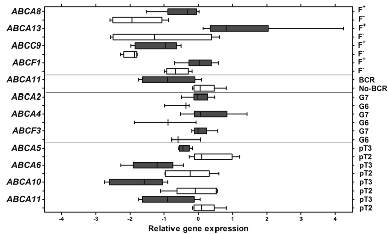
Fig. 2 Significant changes ( p < 0.05 ) of ABC transporter gene expression in PCa according to selected variables. F^{+/-} – TMPPRS2-ERG fusion status; BCR – biochemical recurrence; G7/6 – Gleason score 7/6; pT3/2 – pathological tumor stage 3/2. The box extends from the 25 th to the 75 th percentiles. The line in the middle of the box is plotted at the median. The whiskers indicate the smallest and largest values
