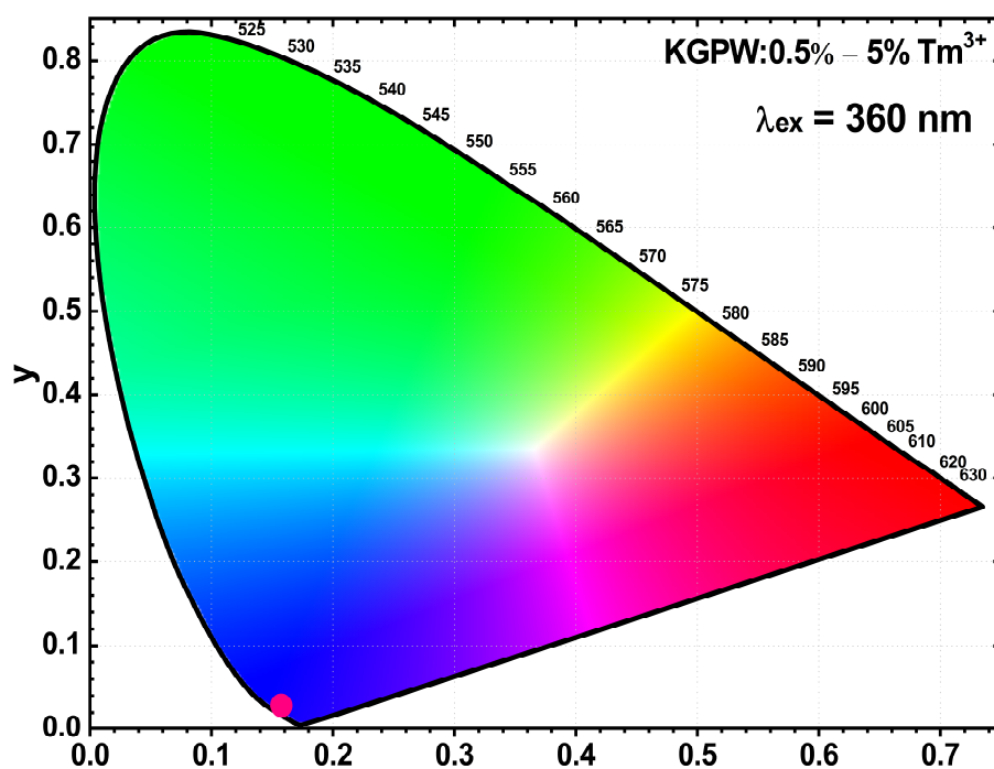
Figure S3. CIE 1931 color space diagram and color coordinates of KGPW:Tm 3+ as a function of Tm 3+ concentration under 360 nm excitation.
