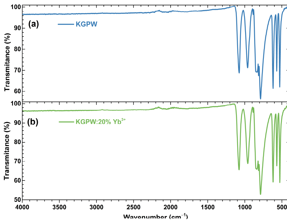
Figure S2. IR spectra of (a) undoped KGPW and (b) KGPW:20%Yb 3+ .
