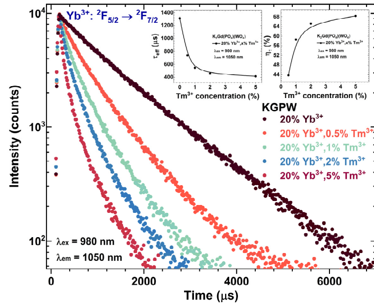
Figure 9. \text{Tm}^{3+} concentration-dependent PL decay curves of \text{Yb}^{3+} in \text{KGPW}:20\%\text{Yb}^{3+},\text{Tm}^{3+} compounds. The inset graphs show \text{Tm}^{3+} concentration-dependent \tau_{\text{eff}} and \eta_{\text{tr}} values.
