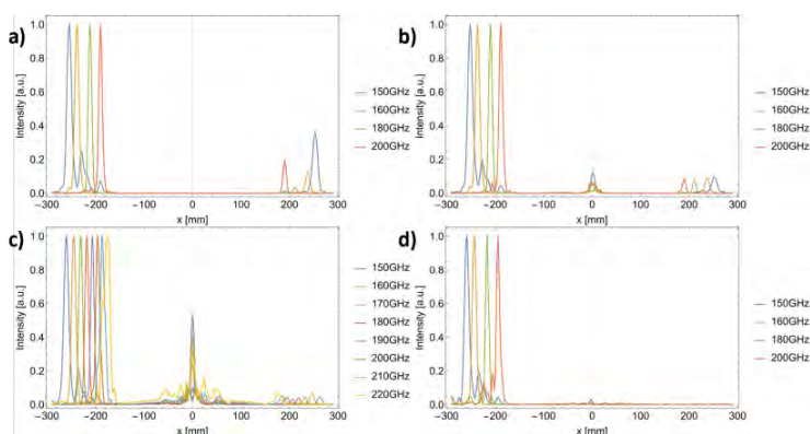
Fig.2 Experimental results for four SIMO structures demonstrating horizontal cross-section of intensity distribution along -1 st , 0 th , and 1 st diffraction order for different THz frequencies. Presented data corresponds to Fig. 1 structures respectively.
