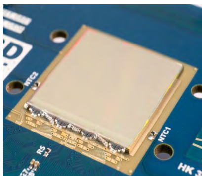
Fig. 1. RD53B chip on single chip test card [3].
