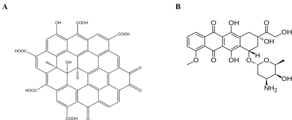
Fig. 1. Chemical structure of graphene quantum dots (A) and doxorubicin (B).
