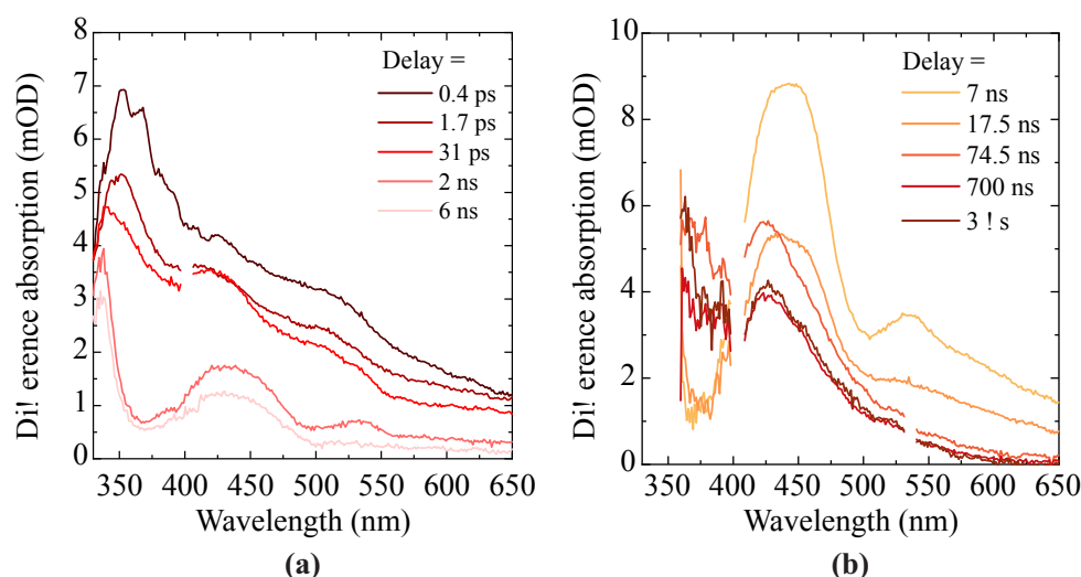
Fig. 1. Transient absorption spectra of BAPO photoinitiator obtained during the (a) pump-probe and (b) laser flash photolysis experiments.
