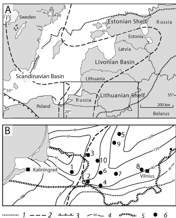
Fig. 2. A, major palaeogeographic features of the Baltic Basin (after Harris et al. 2004). B, localities of drill core sections with described brachiopods: 1, Nesterov-1; 2, Pajevonys-13; 3, Jurbakas-36; 4, Kalvariija-2; 5, Krekenava-7; 6, Sasnava-6; 7, Prienai-3; 8, Vilnius (Griškekes)-1; 9, Ledai-179; 10, Sutkai-89. Legend: 1, outer limit of the distribution of Ordovician deposits; 2, boundary between main facies belts; 3, Caledonian front; 4, isopachs (m) (Paškevičius 1997); 5, administrative boundary; 6, drill core.
