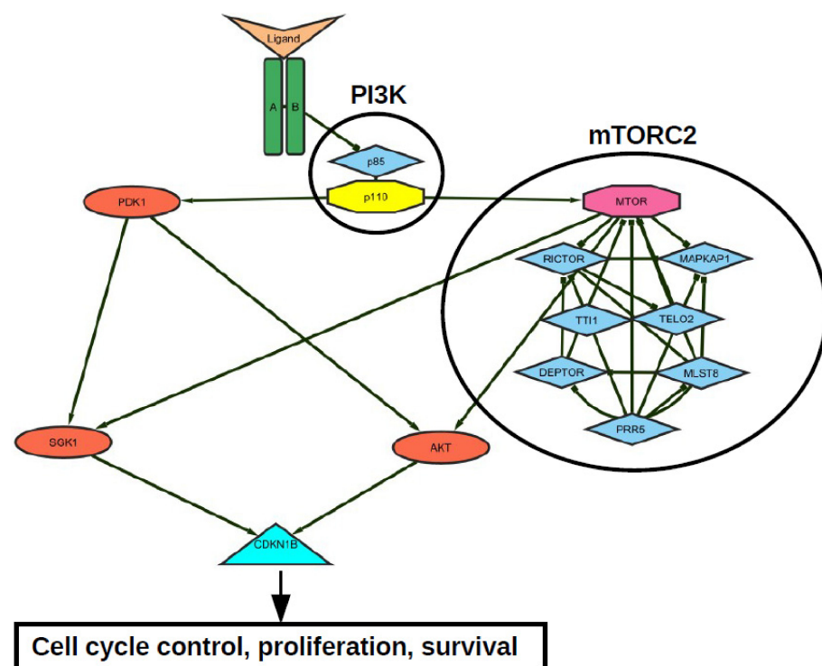
Figure 2. Representative receptor tyrosine kinase—mTORC2—PI3K—AKT—SGK1 signal network. Both AKT- and SGK-mediated CDKN1B (p27) T157 phosphorylation opposes p27-mediated G1 arrest and thus increases proliferation, survival and tumor growth.
