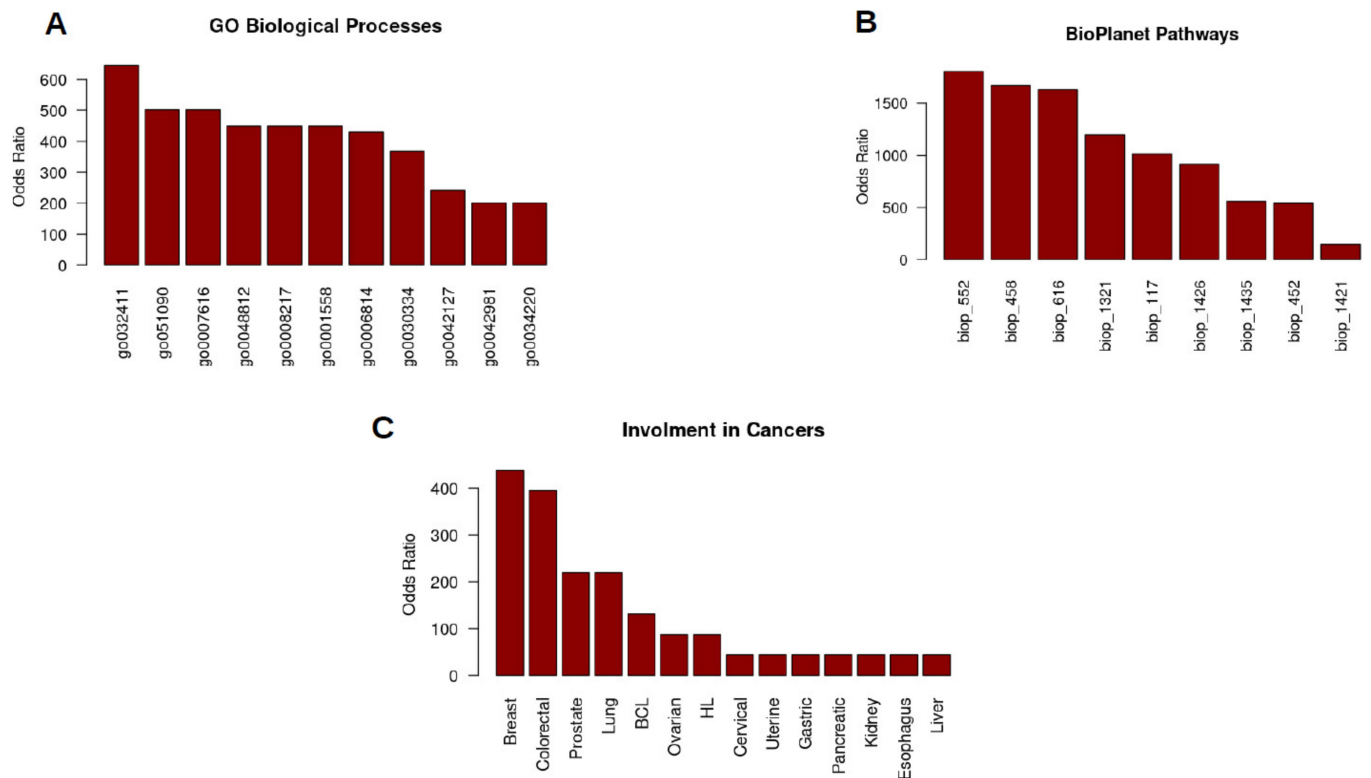
Figure 3. Involvement of SGK1 in major processes and cancers. (A) Most significant gene ontology biological processes in which SGK1 is involved. Positive regulation of transporter activity GO:0032411, regulation of DNA-binding transcription factor activity GO:0051090, long-term memory GO:0007616, neuron projection morphogenesis GO:0048812, regulation of blood pressure GO:0008217, regulation of cell growth GO:0001558, sodium ion transport GO:0006814, regulation of cell migration GO:0030334/ regulation of cell population proliferation GO:0042127, regulation of apoptotic process GO:0042981, ion transmembrane transport GO:0034220. (B) Involvement of SGK1 in most significant signaling pathways, calculated using BioPlanet data. FSH signaling pathway bioplanet_552, aldosterone-regulated sodium reabsorption, bioplanet_458, FoxO family signaling bioplanet_616, regular glucocorticoid receptor pathway bioplanet_1321, mTOR signaling pathway bioplanet_117, interleukin-5 regulation of apoptosis bioplanet_1426, FSH regulation of apoptosis bioplanet_1435, insulin signaling pathway bioplanet_452, interleukin-2 signaling pathway, bioplanet_1421. (C) Most studied types of malignant diseases with a SGK1 playing certain role. Analyzed by biostatistics/bioinformatics at MAP Kinase Resource using data curated at Swiss Institute of Bioinformatics (Geneva, Switzerland) (Jonas Cicenias).
