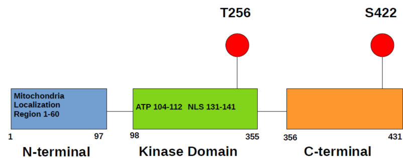
Figure 1. SGK1 domain structure. There is region necessary for mitochondrial localization in N-terminus and nuclear localization signal (NLS) in kinase domain. Kinase domain also contains ATP binding pocket. Most important activating phosphorylation sites are located in kinase domain and C-terminus.
