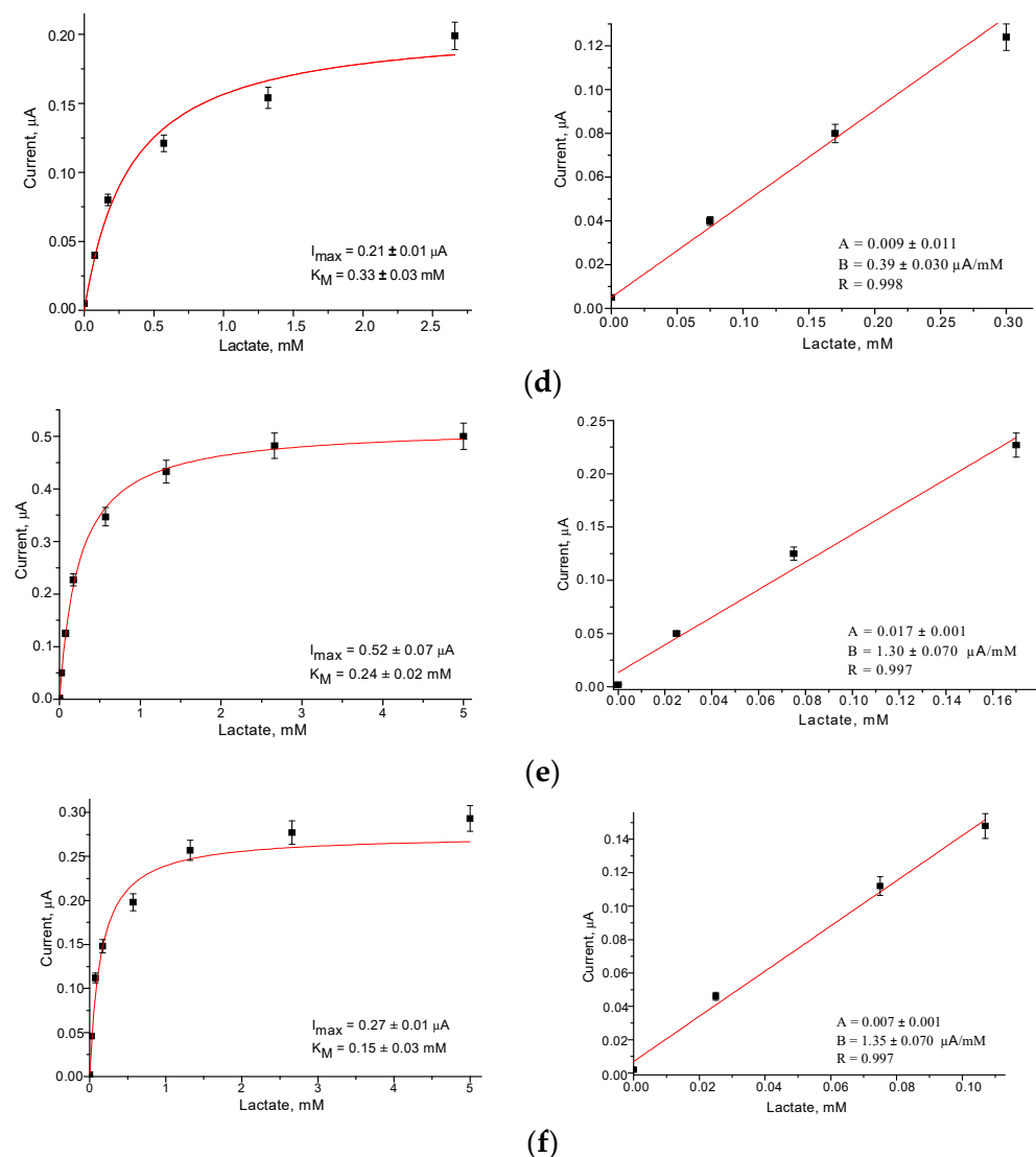
Figure 4. Calibration curves for Lact determination in wide (left) and linear (right) ranges using the Fcb_2 /NPs/GEs: (a) control, without NPs; (b–f) samples with AuHCF (b), PdHCF (c), PtHCF (d), PtZn (e), and NiPtPd (f). Each bioelectrode contained 25 μM of Fcb_2 and 1 μg of NPs on the surface of the GE. Conditions: 50 mM phosphate buffer, pH 8.0, and working potential of -75 mV.
