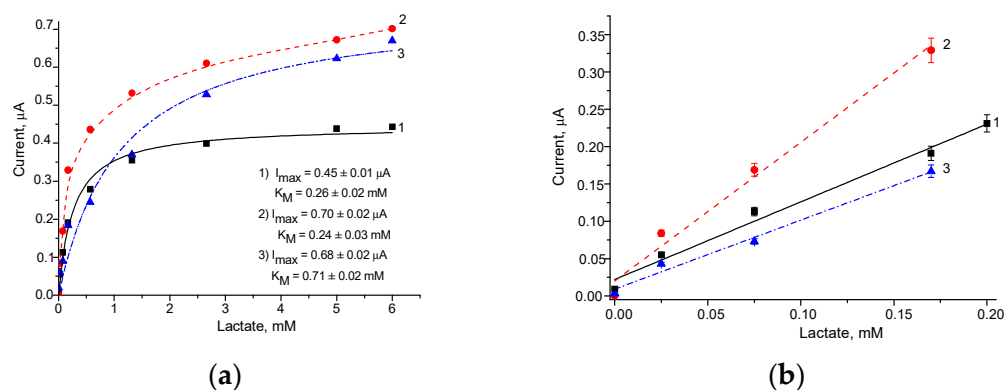
Figure 5. Calibration curves of the Fcb_2/AuHCF/GE s in the broad (a) and linear (b) ranges of the dependence of enzyme quantity on the surface of GE; lines 1, 2, 3 correspond to 13, 25 and 50 mU of Fcb_2 , respectively. The working potential is -75 \text{ mV} .
