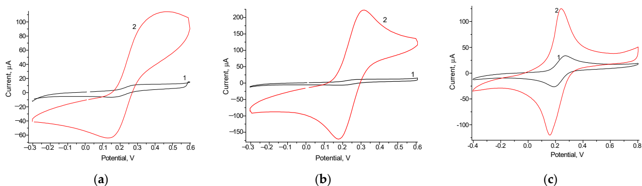
Figure 3. CV profiles of the control GE (a–c, line 1) and the modified electrodes: AuHCF/GE (a, 2), PtZn/GE (b, 2) and gCuHCF/GE (c, 2). Conditions: 10 mM K_3Fe(CN)_6 , 100 mM KCl in 50 mM phosphate buffer, pH 6.5, and 20 °C.
