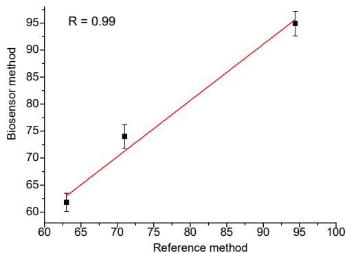
Figure A4. Correlation between the results of the determination of Lact content (mM) in drinking yogurts via reference enzymatic-chemical ( Fcb_2 /PB) and biosensor methods.
