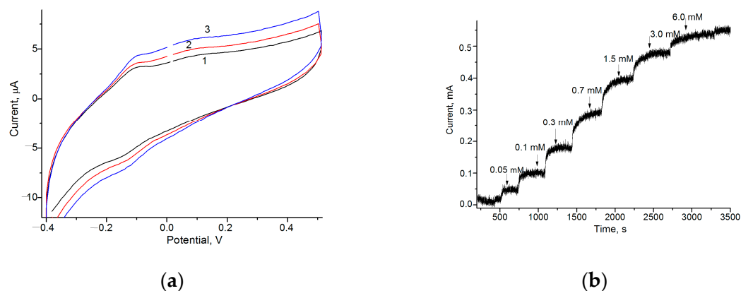
Figure 2. Amperometric characteristics of the Fcb_2/GE as current responses to the increasing concentrations of Lact. (a) CV profiles at Lact concentrations: 0 mM (1, black), 2 mM (2, red), and 5 mM (3, blue); (b) chronoamperogram at the working potential of -75 mV.
