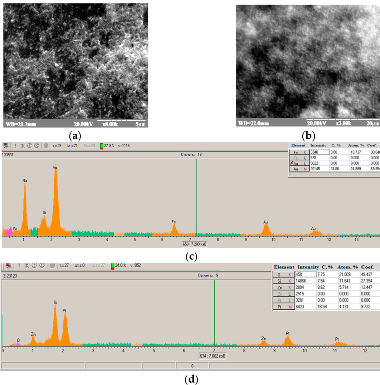
Figure A1. Structural and morphological characterizations of the AuHCF/NPs (a,c) and PtZn/NPs (b,d); the SEM images (a,b) with the correspondent XRM spectra (c,d).
