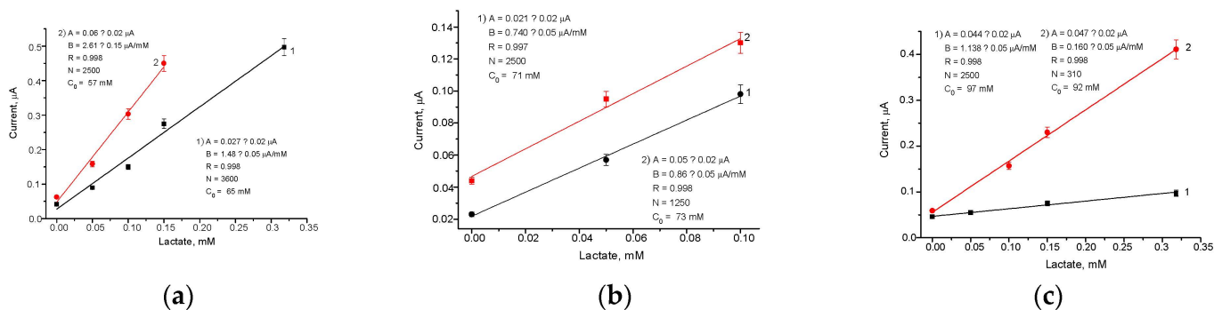
Figure A3. Assay of Lact in the samples of different yogurts (1–3) via graph SAT method (a–c, respectively), using Fcb_2 /AuHCF/GE (25 \mu M Fcb_2 per ABS).
