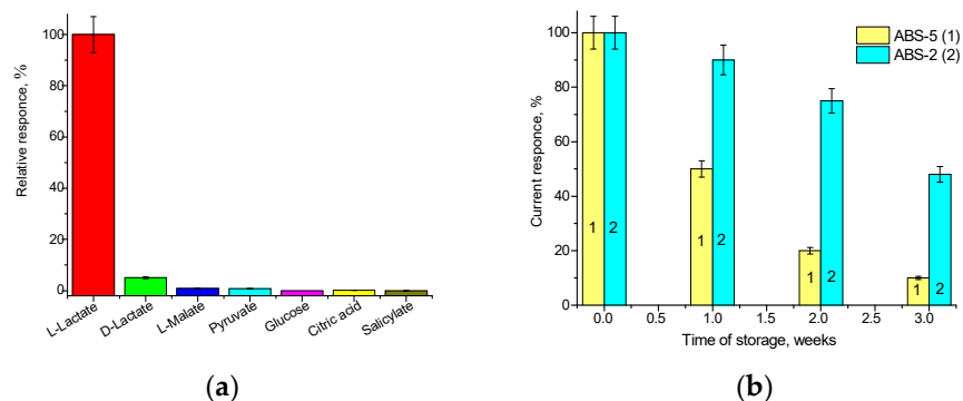
Figure A2. Properties of the Fcb_2 -based ABSs. The selectivity test for AuHCF/GE (ABS-2); current outputs in relative units (%) on the added compounds, up to 2 mM concentration. As a 100% signal, the highest current response on L-Lact was taken (a). Stabilities of the NPs-based ABS-2, and control ABS-5 without NPs (b).
