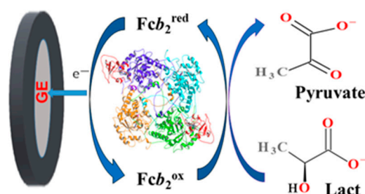
Figure 1. The principal scheme of Lact determination using the Fcb 2 -based ABS.
