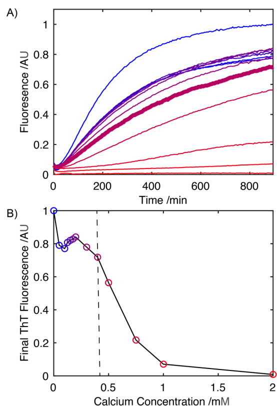
Figure 1. Influence of \text{Ca}^{2+} on the kinetics of S100A9 ( 3.3 \text{ mg mL}^{-1} ) Thioflavin-T positive fibril formation in 20 mM Tris buffer (pH 7.2) (A). Fibril formation was monitored at 0, 0.05, 0.10, 0.125, 0.15, 0.175, 0.20, 0.30, 0.40, 0.50, 0.75, 1.00 and 2.00 mM concentrations of \text{Ca}^{2+} ions (concentration of \text{Ca}^{2+} ions increasing from blue to red, with colouring matching the data points in (B)). The concentration at which S100A9 aggregation starts to be suppressed significantly by \text{Ca}^{2+} , 0.4 mM is highlighted in bold (A). Corresponding plot of Thioflavin-T fluorescence at the plateau level after S100A9 incubated at 41 °C for 15 h, highlighting the drop in total amount of S100A9 fibrils formed as the \text{Ca}^{2+} concentration is increased (B). Vertical line (in (B)) represents the concentration at which the \text{Ca}^{2+} ions begin to suppress the S100A9 aggregation (data point corresponds to the trace in bold in (A)).
