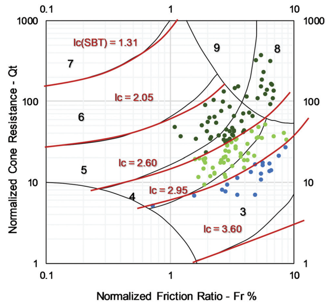
Fig. 4 Distribution of the investigated Pleistocene glacial till soils in P.K. Robertson's (2016) soil behaviour type graph with the indicated I_C soil behaviour type boundaries: 3 – clays, 4 – silt mixture, 5 – sand mixture, 6 – sands, 7 – gravelly sand, 8 – very stiff sand to clayey sand, 9 – very stiff fine-grained sand
