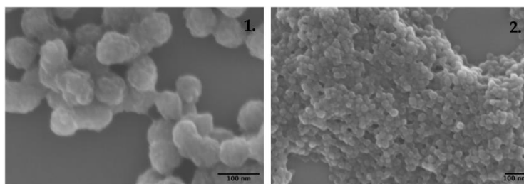
Figure 1. SEM images of (1) PANI and (2) PPy nanoparticles.
