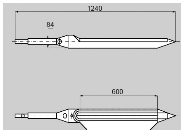
2 pav. Grunto ėmiklis su apsaugine sklende Fig. 2. Sediment sampler with safety valve
