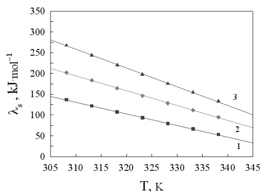
Fig. 4. Dependence of solvent reorganization energy during the electrocatalytic reduction of water clusters on the binary alloys Co-Mo (■ – 1), Ni-Mo (◆ – 2) and Fe-Mo (▲ – 3) in a 30 wt. % NaOH solution on temperature
