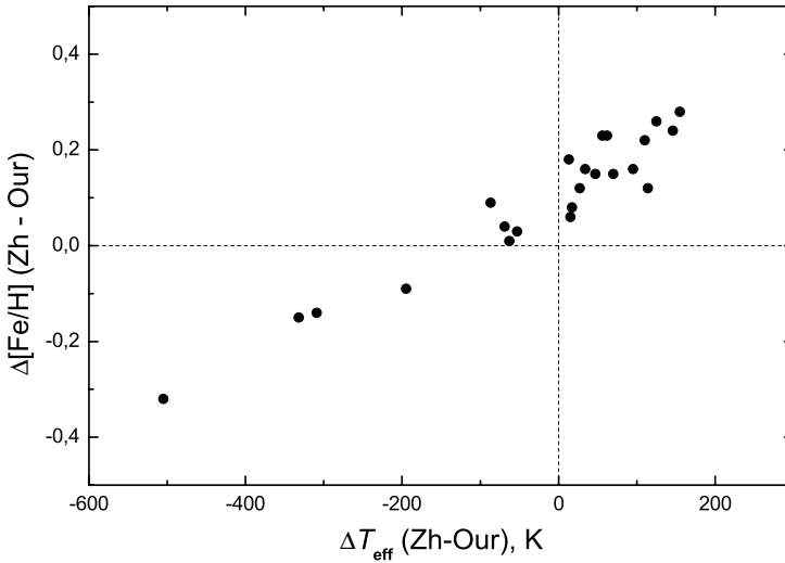
Figure 3.1. The differences of temperature and metallicity caused by the erroneous temperature calibration used by Zhao et al. (2001).
