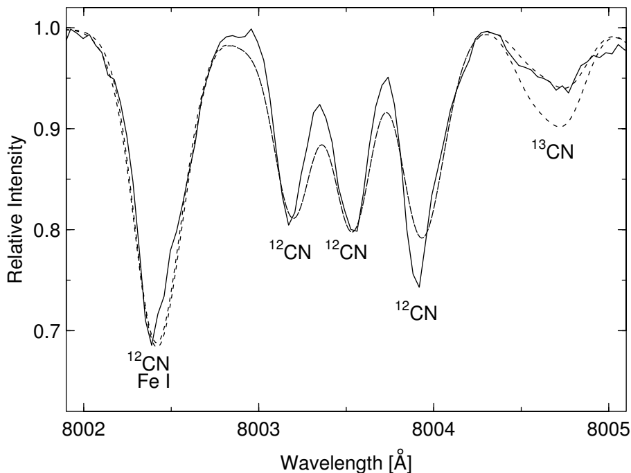
Figure 2.3. Stellar spectrum synthesis example around CN lines in HD2910. The solid line shows the observed spectrum and the dashed lines show the synthetic spectra generated with ^{12}\text{C}/^{13}\text{C} equal to 20 (upper line) and 10 (lower line).
