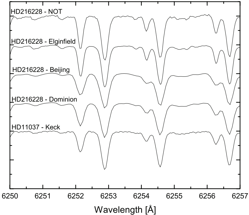
Figure 1.4. The spectrum of the star HD 216228 in the region 6250 to 6257 Å as observed on four different telescopes. Since this star was not observed on the Keck telescope, we present a spectrum of the very similar star HD 11037 instead.
