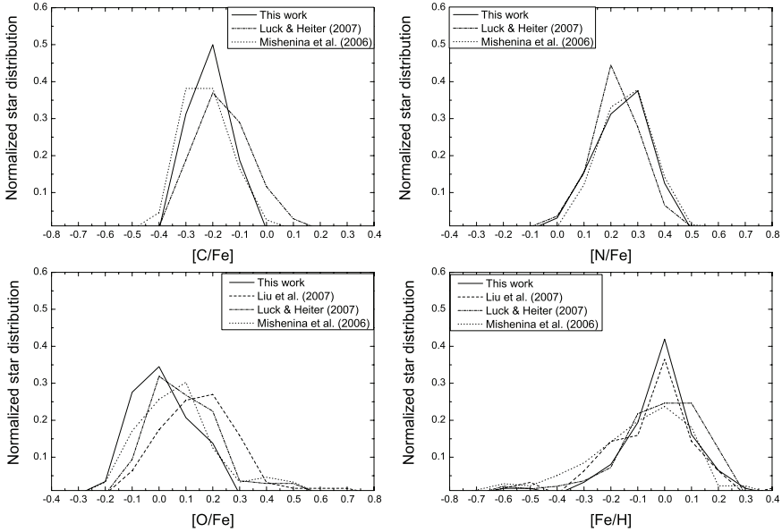
Figure 4.3. C, N, O and [Fe/H] abundance distributions in the samples of Galactic clump stars investigated in this dissertation, by Mishenina et al. (2006), by Liu et al. (2007) and by Luck & Heiter (2007).
