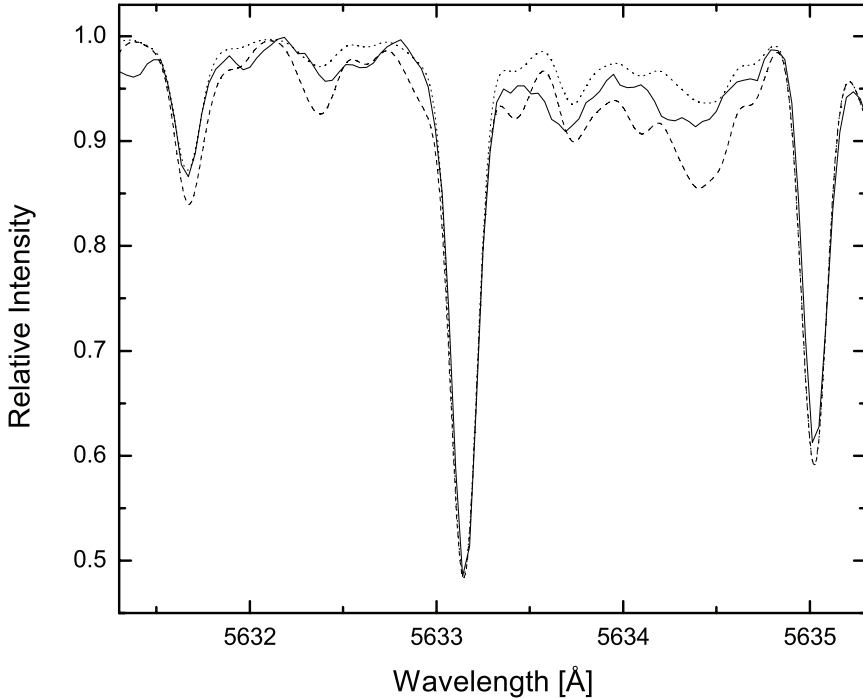
Figure 2.2. Synthetic and observed spectra for the C 2 region near 5635 Å of HD 8763. The solid line shows the observed spectrum and the dotted and dashed lines show the synthetic spectra generated with [C/Fe] = 0 and -0.2
