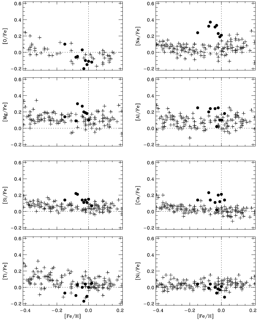
Figure 5.2. Element to iron ratios as a function of iron [\text{Fe}/\text{H}] . Results of this dissertation paper are indicated by filled circles, results obtained for dwarf stars of the galactic disk (Edvardsson et al. 1993) by '+' signs.
