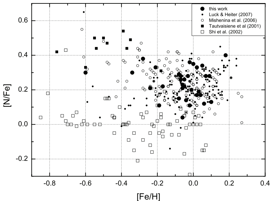
Figure 4.2. [N/Fe] as a function of [Fe/H] . We show the results for the clump stars investigated in this work, in Mishenina et al. (2006) and in Luck & Heiter (2007). Also we show the results obtained for red horizontal branch stars by Tautvaišienė et al. (2001). For the comparison, results obtained for dwarf stars of the Galactic disk (Shi et al. 2002) are presented.
