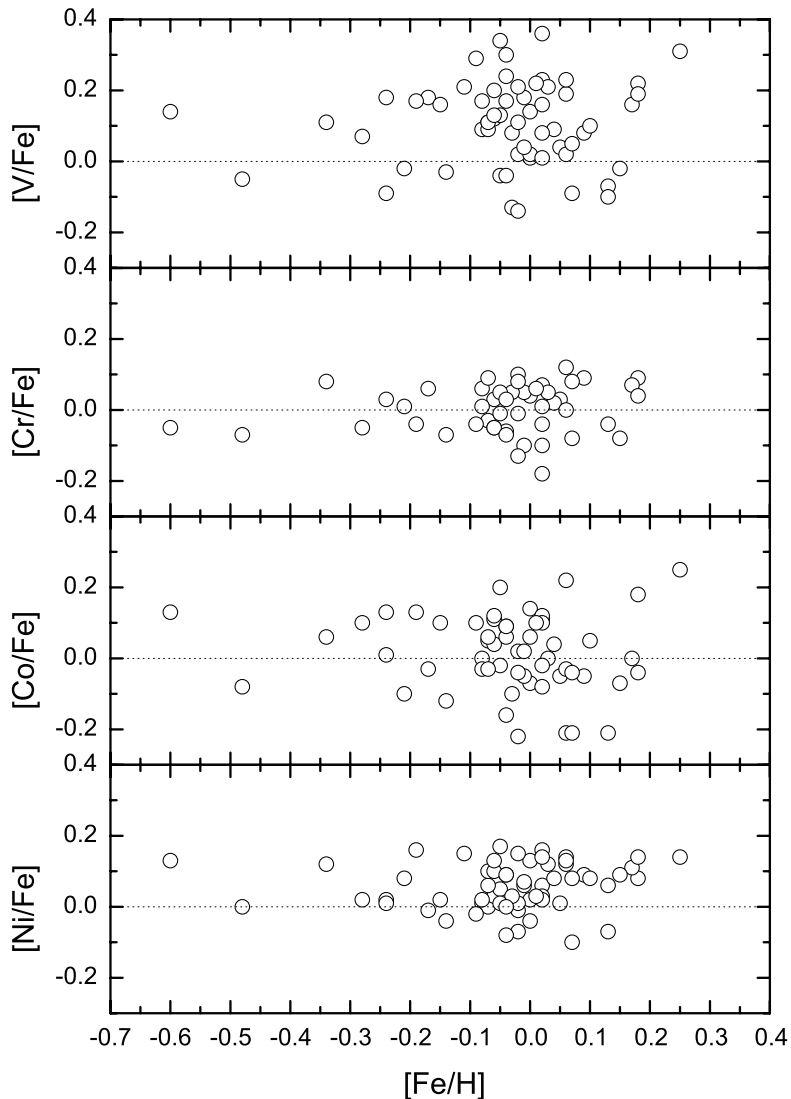
Figure 3.4. Abundance trends of iron group elements.
