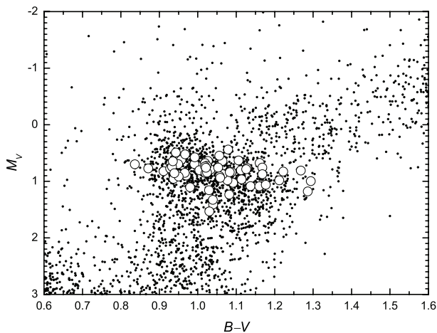
Figure 1.1. Color–magnitude diagram for the Hipparcos catalogue. The programme stars are indicated by open circles.
