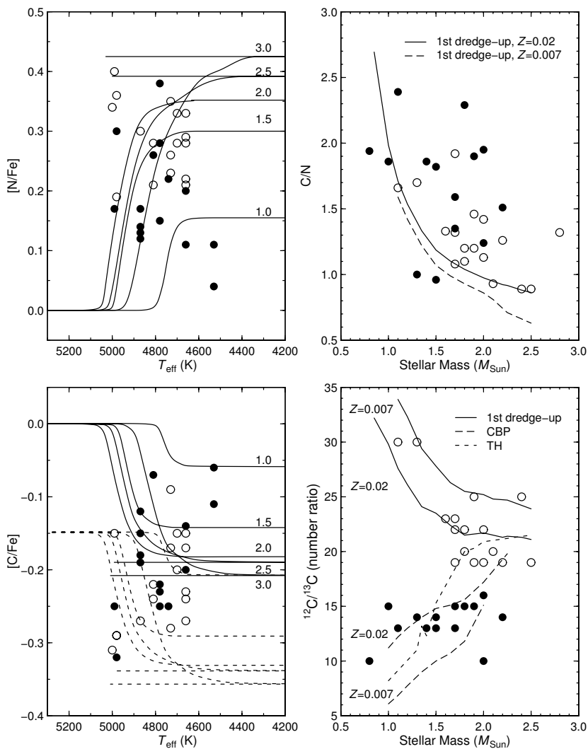
Figure 4.4. On the left side – [\text{C}/\text{Fe}] and [\text{N}/\text{Fe}] versus effective temperatures in the sample of Galactic red clump stars compared with the theoretical tracks of abundance variations taken from Mishenina et al. (2006). The theoretical [\text{C}/\text{Fe}] (dashed lines) are shifted by -0.15 dex (following Mishenina et al. (2006) in order better to represent the majority of metal-deficient stars investigated. On the right side – \text{C}/\text{N} and ^{12}\text{C}/^{13}\text{C} ratios versus stellar mass. The theoretical curves are taken from Boothroyd & Sackmann (1999) – solid and long dashed lines and Lagarde & Charbonnel (2009) – short dashed line. The stars identified as first ascent giants are shown by empty circles, and the stars identified as helium-core-burning stars – filled circles.
