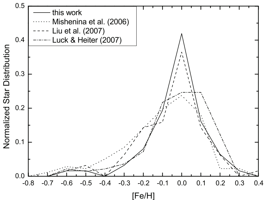
Figure 3.2. Distributions of [\text{Fe}/\text{H}] in the Galactic clump stars investigated in this work and other studies.
