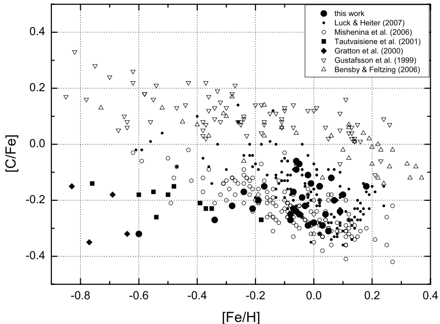
Figure 4.1. Galactic clump abundances: [C/Fe] as a function of [Fe/H] . We show the results for the clump stars investigated in this work, in Mishenina et al. (2006) and in Luck & Heiter (2007). Also we show the results obtained for red horizontal branch stars by Tautvaišienė et al. (2001) and by Gratton et al. (2000). For the comparison, results obtained for dwarf stars of the Galactic disk (Gustafsson et al. 1999 and Bensby & Feltzing 2006) are presented.
