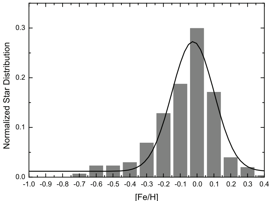
Figure 3.3. Metallicity distribution in the sample of 342 Galactic clump stars (the [\text{Fe}/\text{H}] values are averaged for the common stars investigated in this study, Mishenina et al. (2006), Liu et al. (2007) and Luck & Heiter (2007)).
