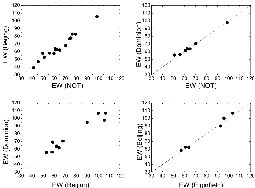
Figure 2.1. Comparisons of equivalent widths of Fe I lines in overlapping spectral regions observed with different telescopes for Galactic clump star HD 216228.
