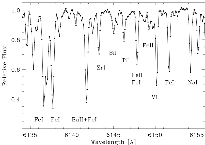
Figure 1.3. Sample spectrum of cluster NGC7789 star K765.
