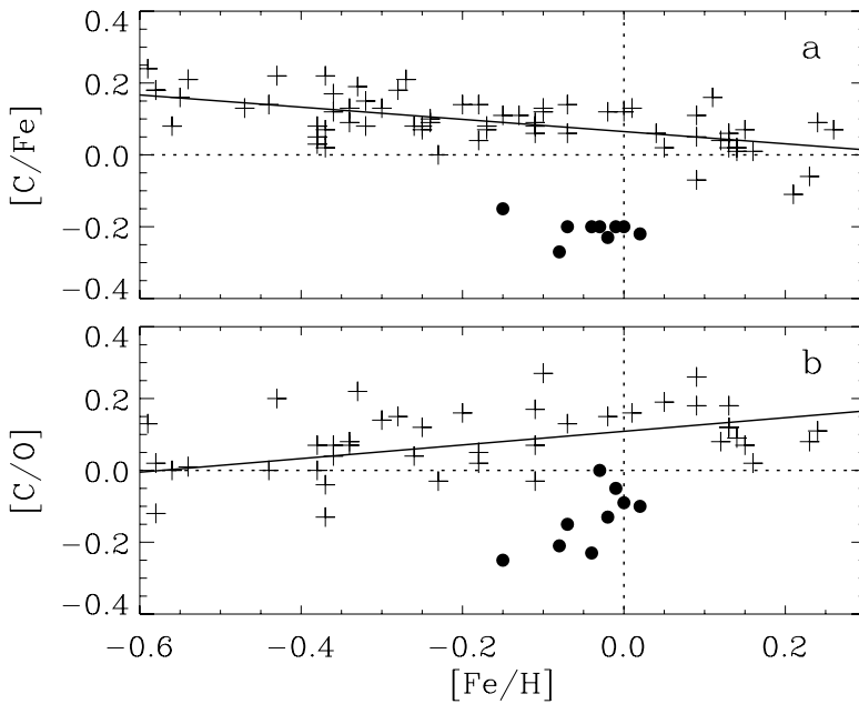
Figure 5.1. [C/Fe] and [C/O] as a function of [Fe/H]. Results of this dissertation are indicated by filled circles, results obtained for dwarf stars of the Galactic disk (Gustafsson et al. 1999) by 'plus' signs and the full line.
