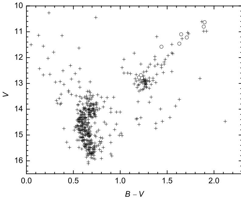
Figure 1.2. The colour–magnitude diagram of the open cluster NGC 7789. The red giants and the core–He–burning “clump” stars analysed in dissertation are indicated by the open circles. The diagram is based on UBV observations by Burbidge & Sandage (1958).
