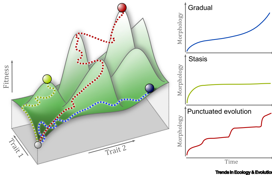
Figure 2. Three agents take adaptive walks on a fitness landscape, starting at the same point. Sewell Wright introduced the metaphor of a fitness landscape to describe the possible mutational trajectories (gradual, stasis, and punctuated) that lineages take (evolve) from genotypes that lie in regions of low fitness to regions of higher fitness. The landscape also contains valleys, which correspond to designs that yield negative fitness. There might be any number of pathways that the agents can take as they move about the landscape, a process that Kauffman et al. [89] referred to as an ‘adaptive walk.’ The model shown here is highly simplified in that it assumes a static landscape, which is rarely the case. Rather, the actions of other agents are constantly affecting the landscape, creating what Kauffman referred to as a ‘dynamic fitness landscape’ [90].
