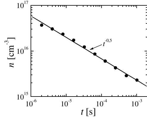
Fig. 18. Photogenerated charge carrier density as a function of time measured using photo-CELIV. The line corresponds the t^{-1/2} dependence ( d = 2.6 \mu\text{m} ).
