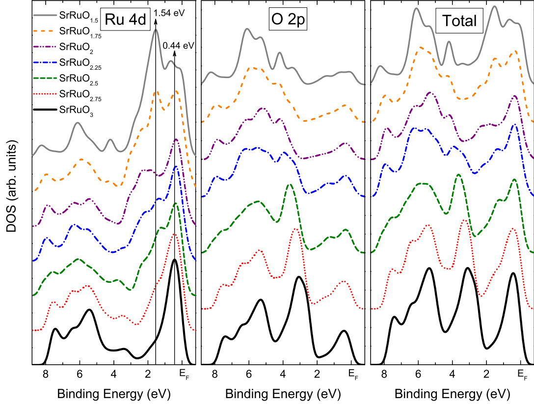
Figure 5.8 The total and projected DOS of \text{SrRuO}_3 after removal of \text{O}_x ( x = 1-6 ) atoms from the unit cell. The calculations were performed with full relaxation of geometry using PBEsol exchange-correlation functional.
