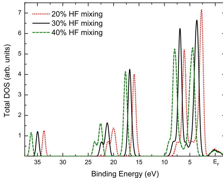
Figure 4.6 The comparison of total DOS of LaNiO 3 calculated within PBE0 framework at different percentage of HF mixing.
