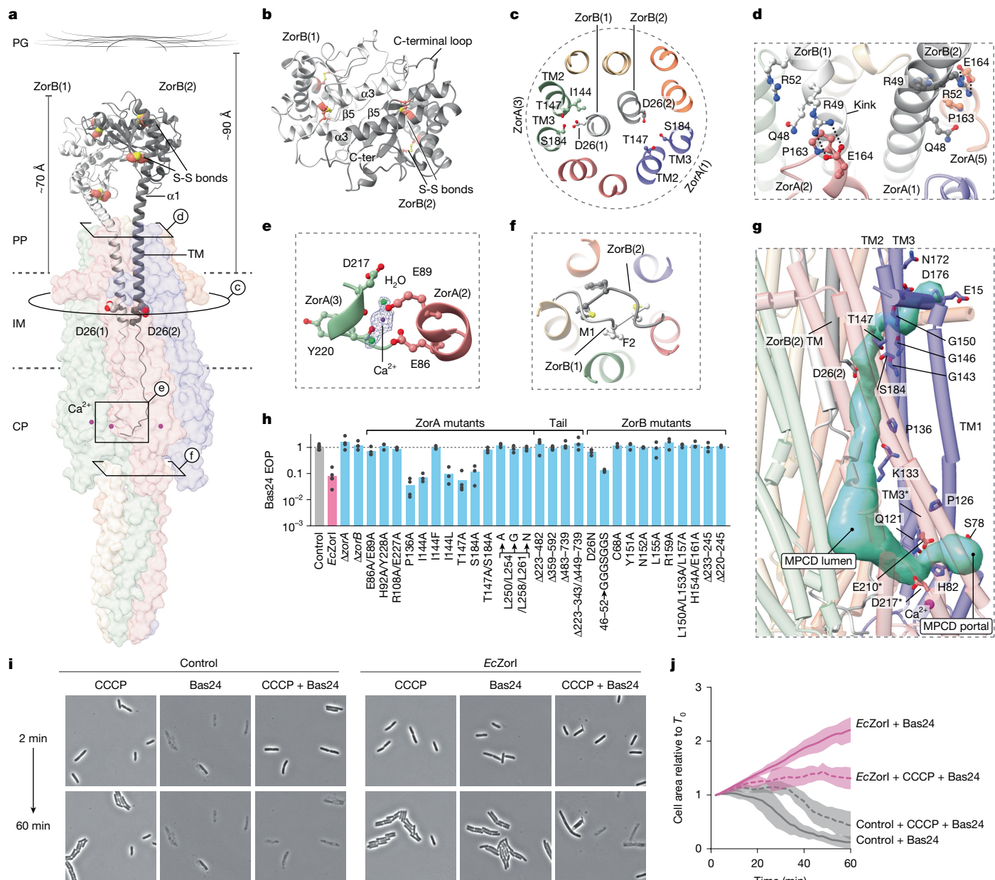
Fig. 3 | ZorAB is a PG-binding, proton-driven motor. a , EcZorAB viewed from the plane of the membrane, with ZorB shown as ribbons (black and white) and ZorA shown as a translucent surface. The distance between the inner membrane and PG layer in E. coli is approximately 90 Å (ref. 32). The cysteine residues from the two disulfide bridges in the ZorB PGBD are indicated and shown as spheres. The Asp26 residues from both ZorB TM helices are indicated and shown. b , Top view of the ZorB PGBD. c , Cross-section view of the ZorAB TMD, showing ZorB Asp26 and the surrounding residues. d , Magnified view of the interactions between ZorB and ZorA at the domain assembly interface in the periplasmic space. e , The \text{Ca}^{2+} -binding site. EM densities are only overlapped on \text{Ca}^{2+} ion, and the two water molecules. f , Magnified view of the interactions between the ZorB N terminus and the ZorA tail. g , Ion-translocation pathway (semitransparent surface representation in light blue) in ZorAB. Residues along the ion-permeation
