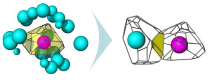
Figure 1. Constructing contact area of two atoms by Voronoi tessellation.
