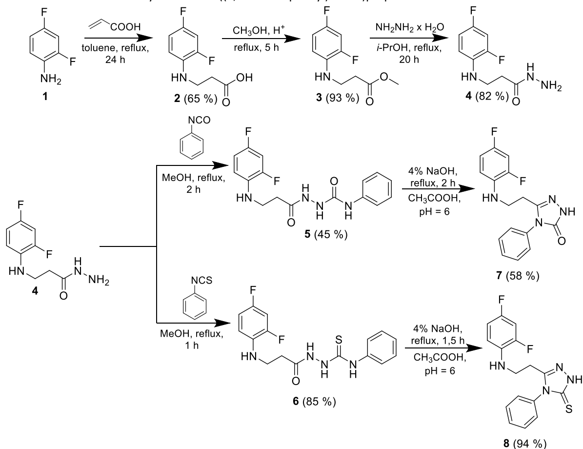
Scheme 1. Synthesis of 3-((2,4-difluorophenyl)amino)propanoic acid derivatives
