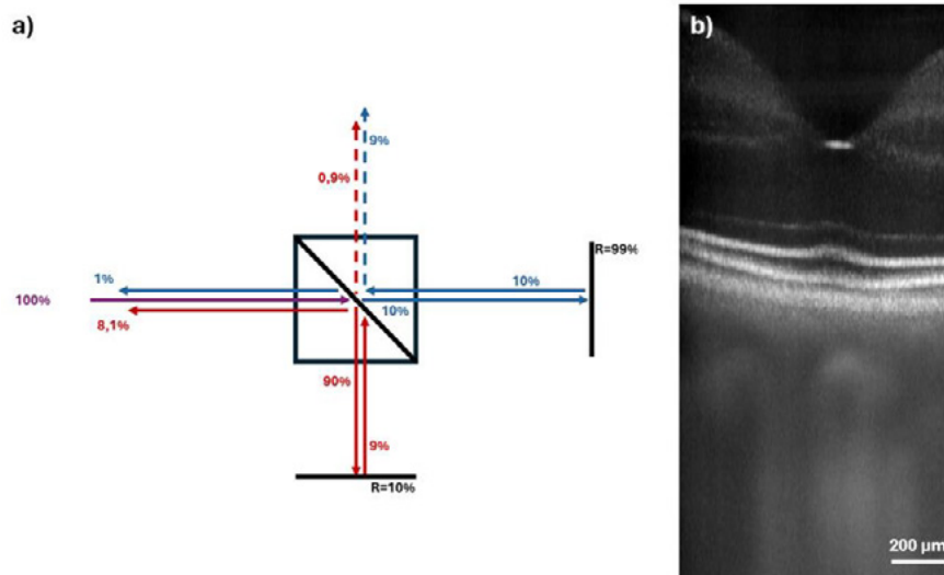
Figure 1. a) – 90/10 cube beam splitter. b) - FF-FD-OCT image of in vivo human retina registered using 90/10 cube beam splitters.
