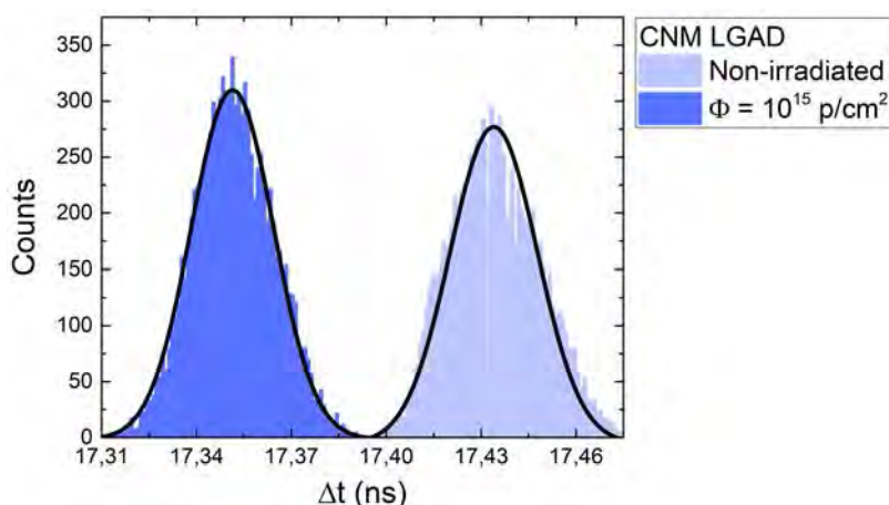
Fig. 1. Comparison of the distributions of time delay between laser pulse and detector signal between non-irradiated and irradiated with protons of fluence 10^{15} \text{ p/cm}^2 samples.
