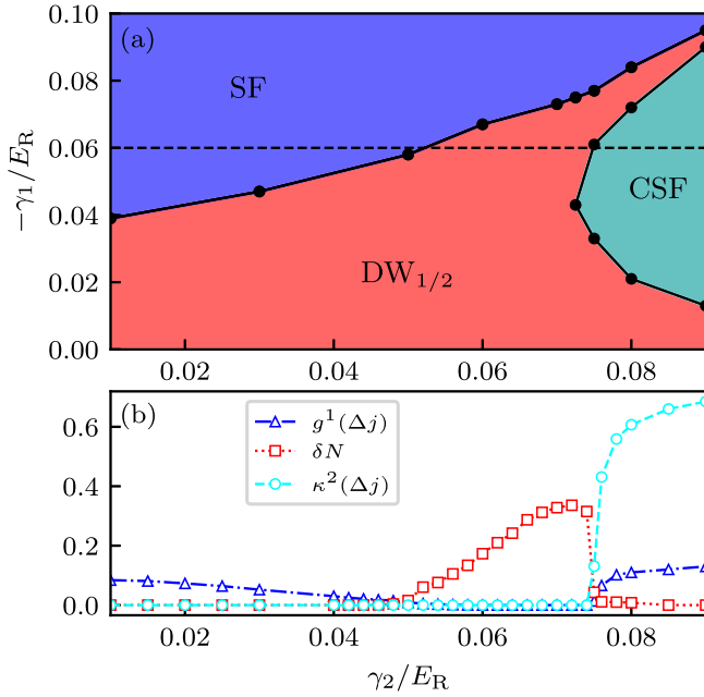
Fig. 6 | Extended Bose-Hubbard model phase diagram and extracted values of Eqs. (15)-(18). Both subplots were computed for N=5 internal states at \bar{n} = 1/2 filling, Raman coupling \Omega/E_R = 3.5 , a system size of L = 181 sites, and 91 particles. a Phase diagram as a function of detuning Fourier components \gamma_1 and \gamma_2 . b Asymptotic correlation functions (one-body Green's function g_{\text{cen}}^{(1)} , staggered density \delta N and asymptotic vector order parameter \kappa_{\text{cen}}^2 ) dependence on \gamma_2 for fixed \gamma_1/E_R = -0.06 , corresponding to the dashed black line in (a).
