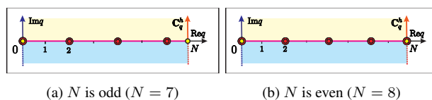
Figure 5. EPs for SLP (39)–(40); \bullet – RP, \circ – simple EP at RP, \bullet – double EP.
