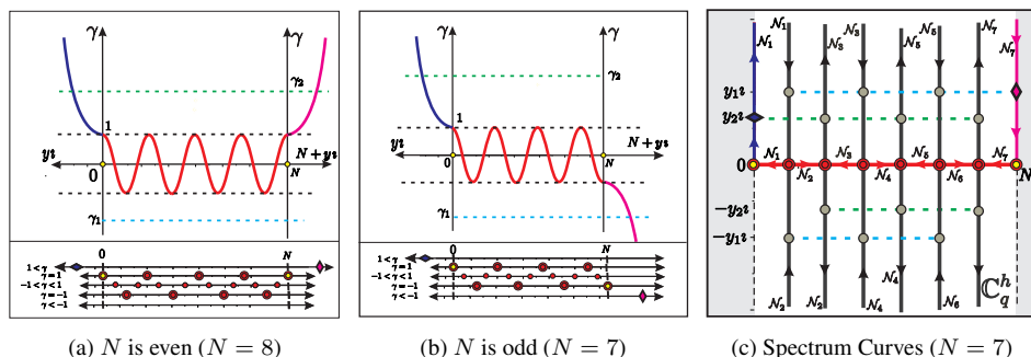
Figure 7. (a), (b) Real CFs (58) and real EPs; (c) EPs in the cases \cosh(\pi y_1) = |\gamma_1| , \gamma_1 < -1 , and \cosh(\pi y_2) = \gamma_2 > 1 , \bullet – complex EP.
