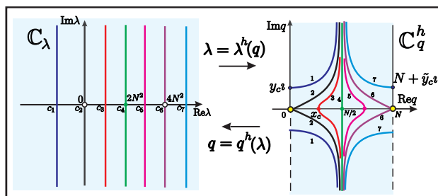
Figure 3. Images of lines \operatorname{Re} \lambda = c_k , k = 1, \dots, 7 , in \mathbb{C}_q^h : c_1 < 0 , c_2 = 0 , 0 < c_3 < 2N^2 , c_4 = 2N^2 , 2N^2 < c_5 < 4N^2 , c_6 = 4N^2 , c_7 > 4N^2 .
