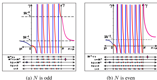
Figure 6. Real CFs (49) and EPs q_k : \square – CEP q_k = c_k , \blacklozenge – large positive EP q_1 = N + y_1 i , \lambda_1 > 4N^2 , \blacklozenge – negative EP q_1 = y_1 i , \lambda_1 < 0 , \bullet – positive EP q_k = x_k , \lambda_k \in (0, 4N^2) .
