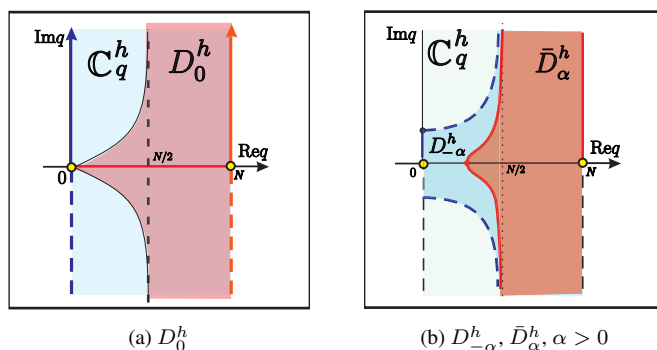
Figure 4. Domains D_0^h, D_{-\alpha}^h, \bar{D}_{\alpha}^h .
