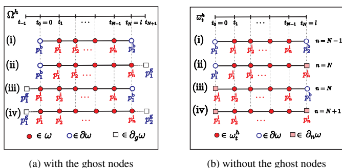
Figure 1. One-dimensional grids \omega , \partial\omega , \partial_g\omega , \omega_t^h , \partial_n\omega ; \square – ghost nodes, \blacksquare – nodes for the natural derivative, \circ – nodes not used by the natural derivative.
