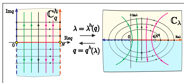
Figure 2. Domain \mathbb{C}_q^h ; \bullet – ramification points q = 0, N , \circ – branch points \lambda = 0, 4N^2 .
